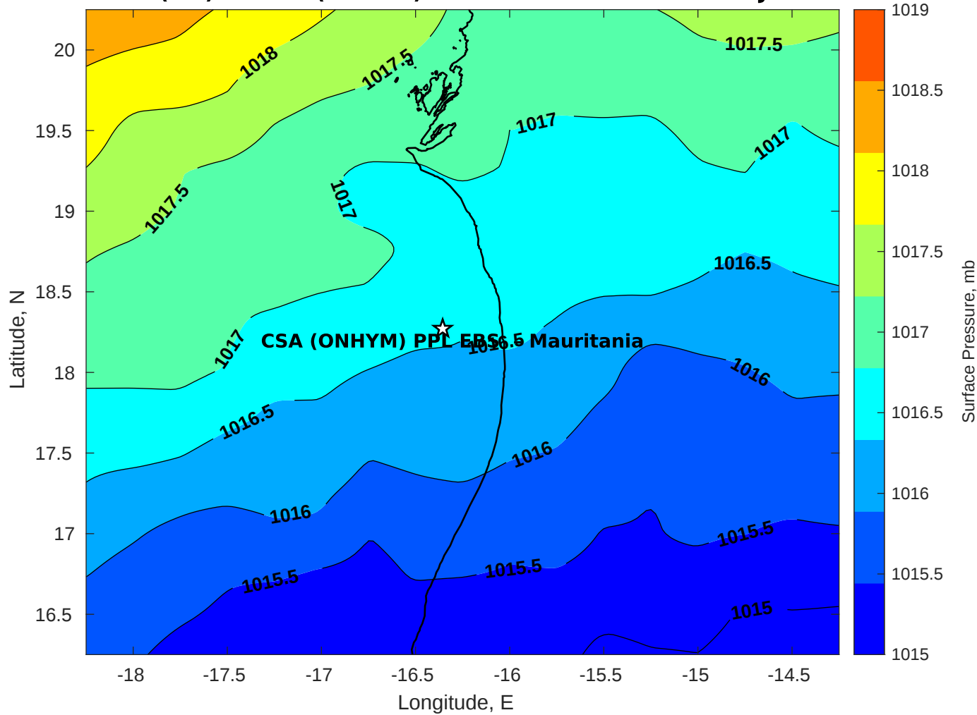
Surface Pressure (mb) for CSA (ONHYM) PPL EBS - Mauritania at 23-Jan-2026 00:00:00
