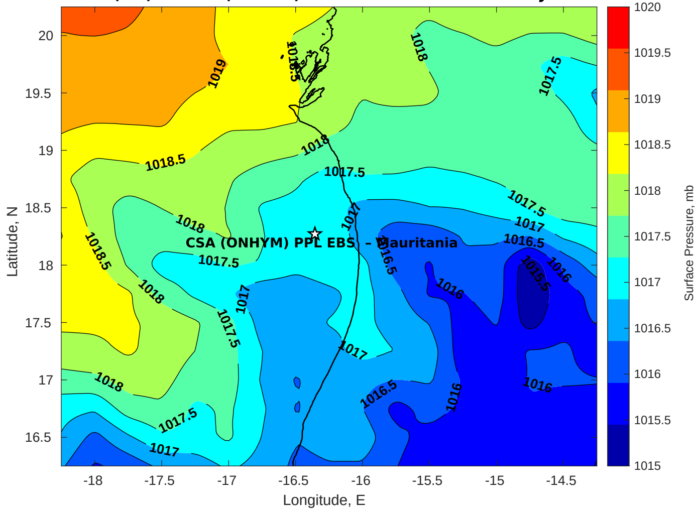
Surface Pressure (mb) for CSA (ONHYM) PPL EBS - Mauritania at 24-Jan-2026 00:00:00
