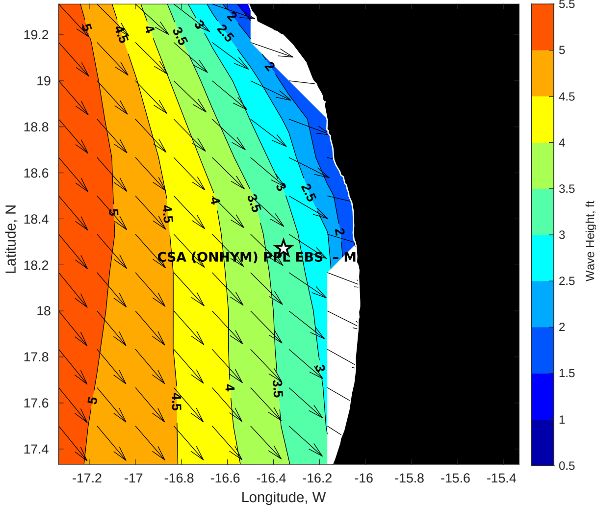
GFS Wave Height (ft) for CSA (ONHYM) PPL EBS - Mauritania at 23-Jan-2026 09:00:00
