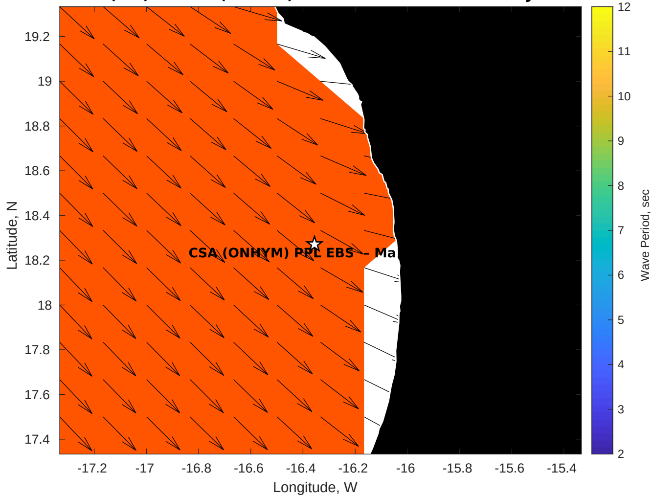
GFS Wave Period (sec) for CSA (ONHYM) PPL EBS - Mauritania at 23-Jan-2026 09:00:00
