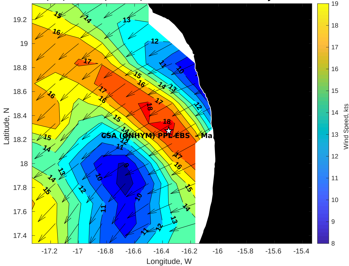
GFS Winds (kts) for CSA (ONHYM) PPL EBS - Mauritania at 23-Jan-2026 09:00:00
