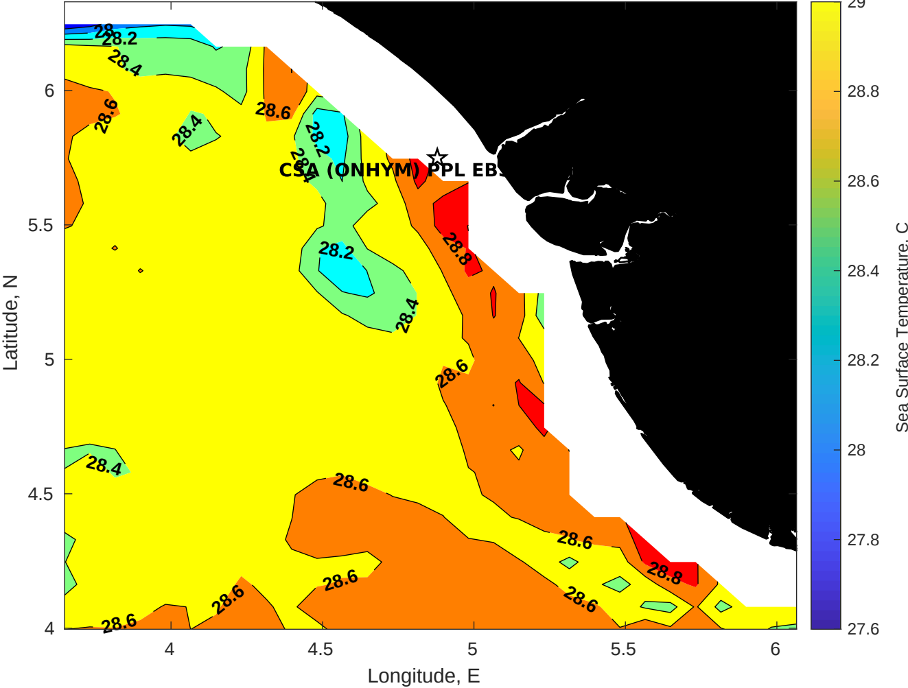
SST for CSA (ONHYM) PPL EBS - Nigeria at 22-Jan-2026 00:00:00
