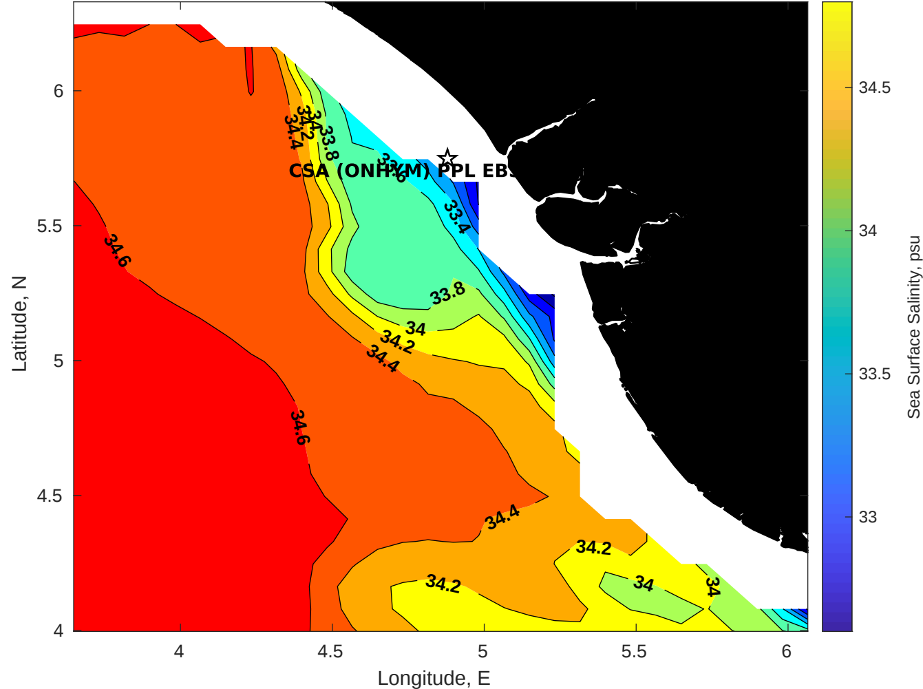
Surface Salinity for CSA (ONHYM) PPL EBS - Nigeria at 22-Jan-2026 00:00:00
