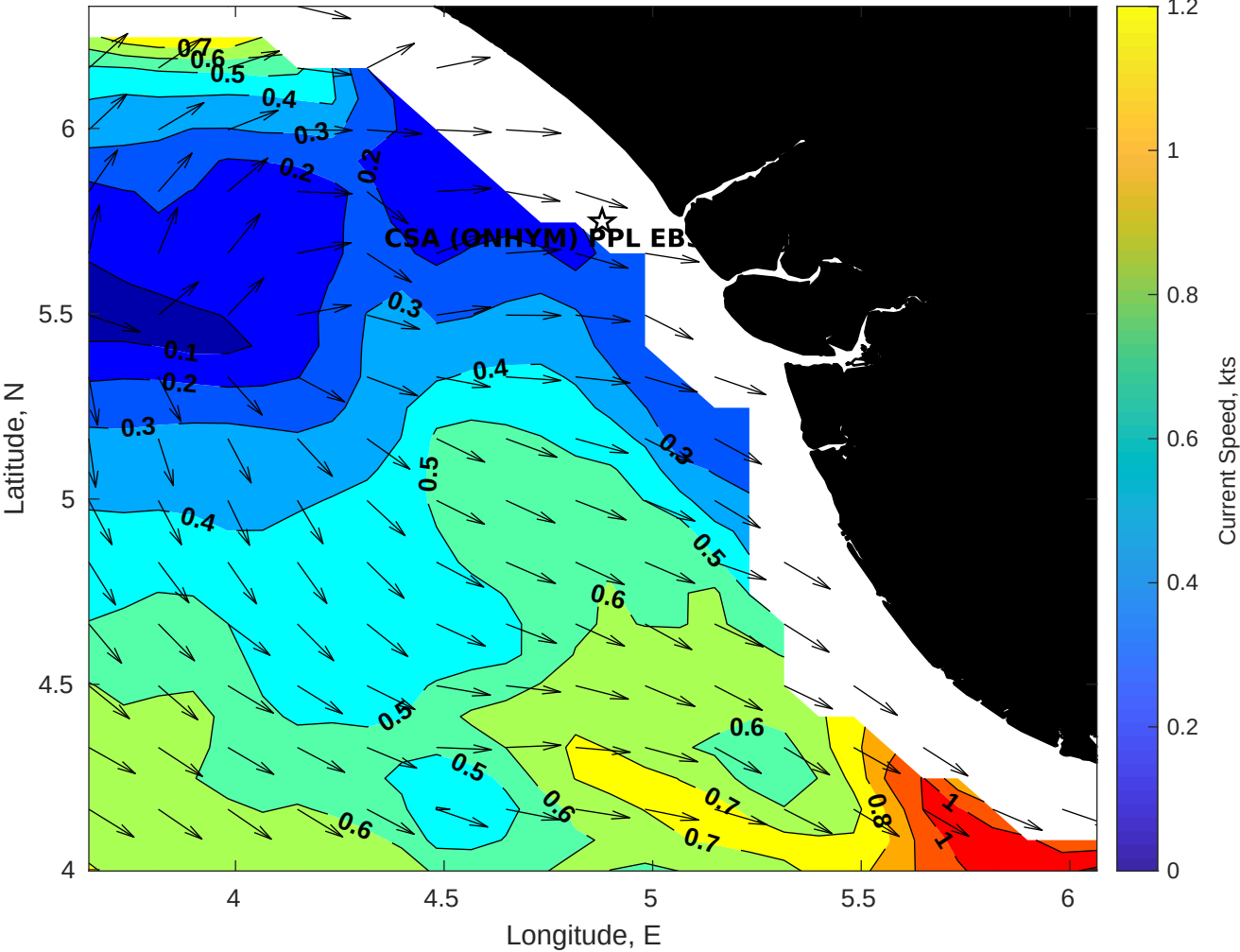
Surface Currents for CSA (ONHYM) PPL EBS - Nigeria at 22-Jan-2026 00:00:00
