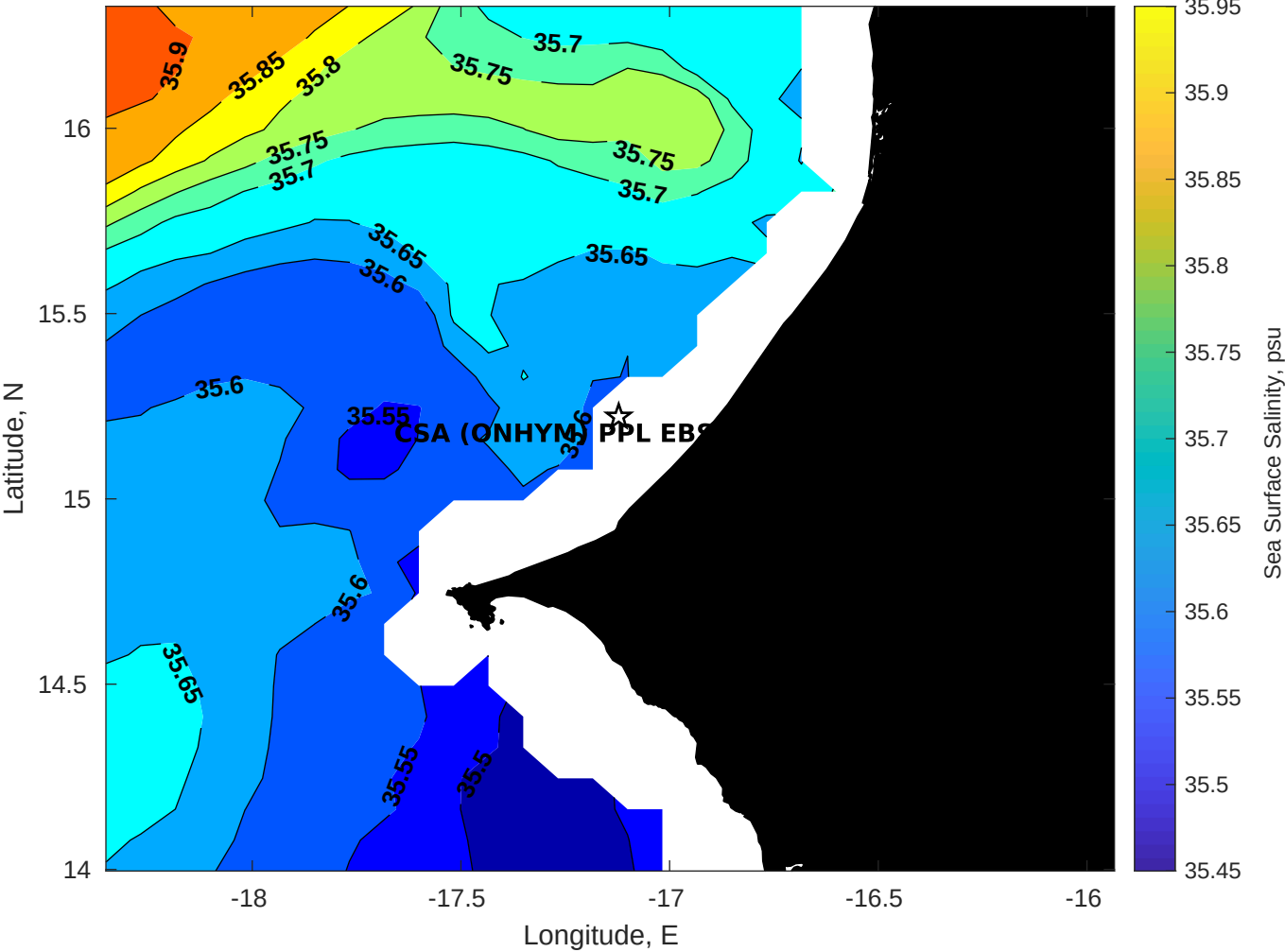
Surface Salinity for CSA (ONHYM) PPL EBS - Senegal at 22-Jan-2026 00:00:00
