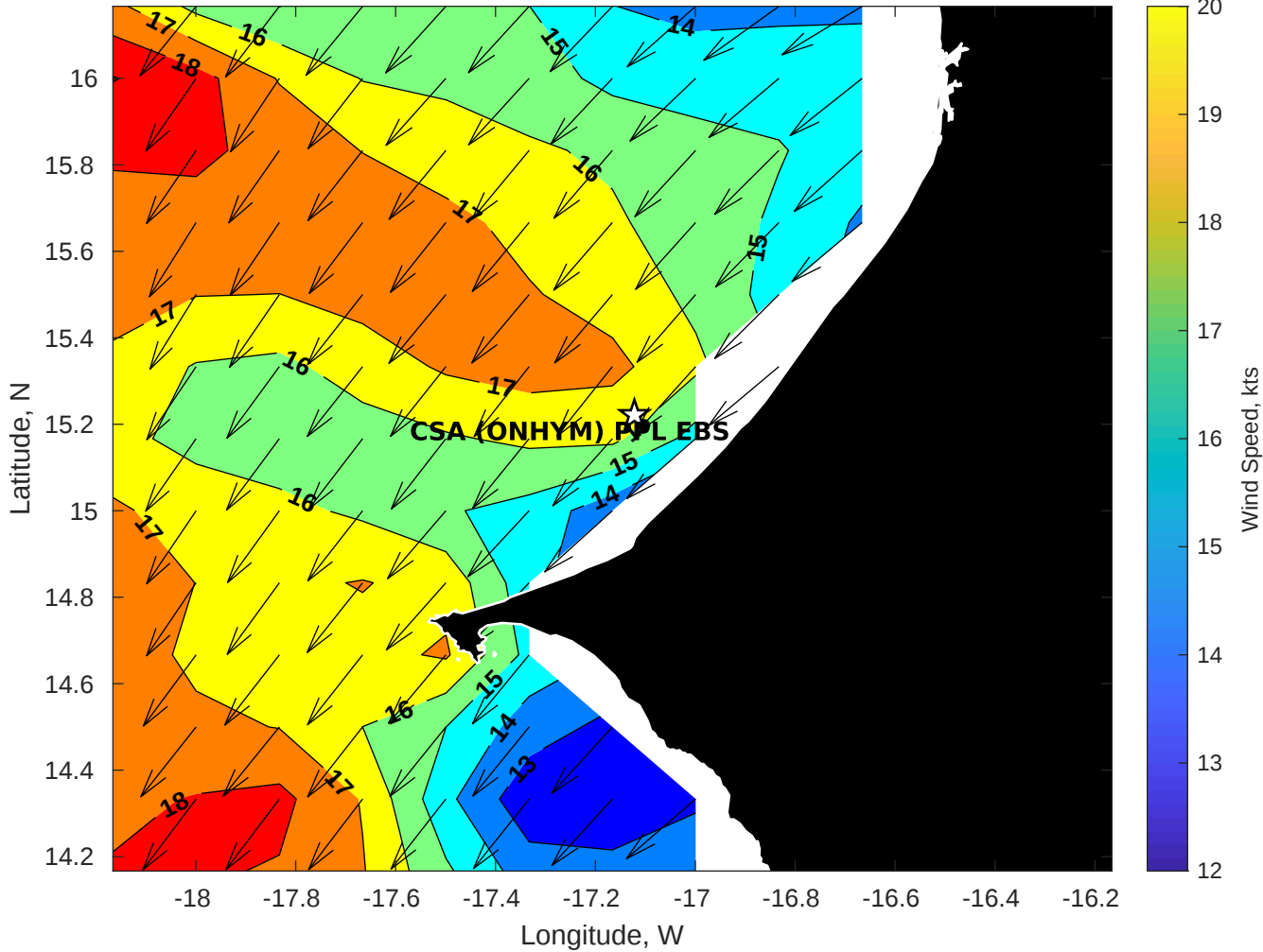
GFS Winds (kts) for CSA (ONHYM) PPL EBS - Senegal at 23-Jan-2026 09:00:00
