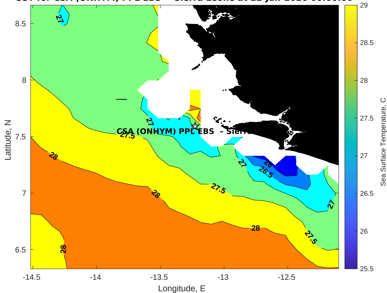
SST for CSA (ONHYM) PPL EBS - Sierra Leone at 22-Jan-2026 00:00:00
