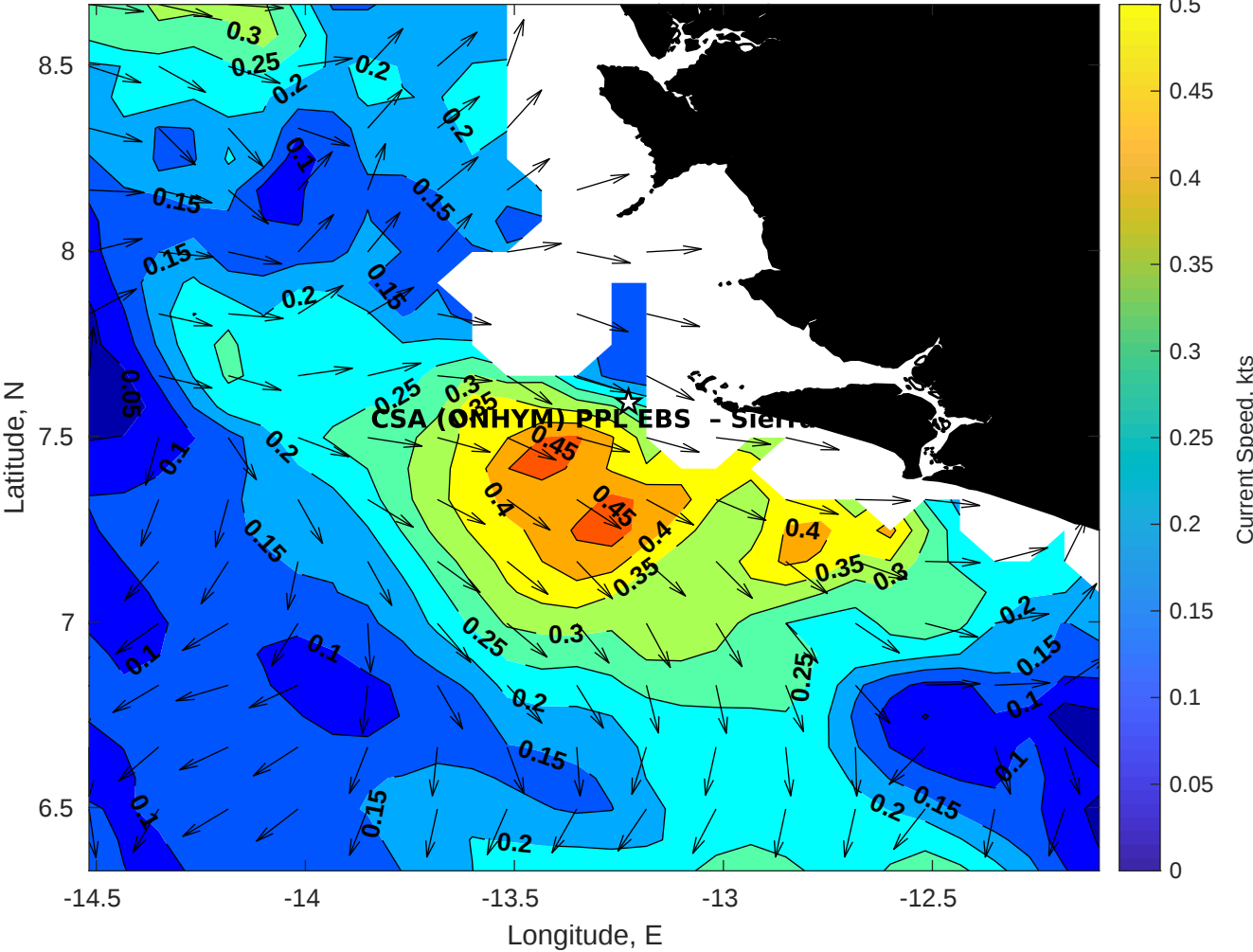
Surface Currents for CSA (ONHYM) PPL EBS - Sierra Leone at 22-Jan-2026 00:00:00
