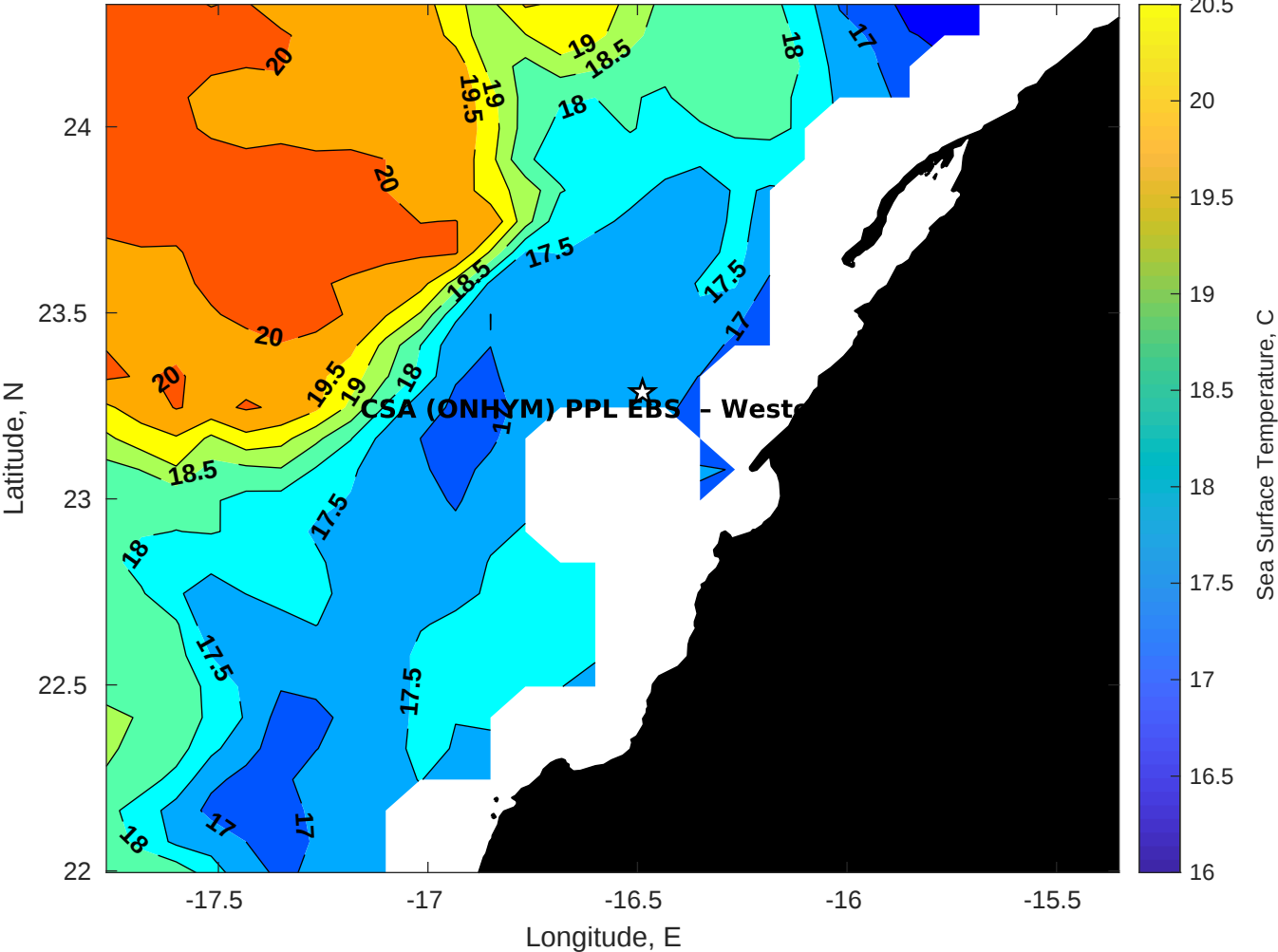
SST for CSA (ONHYM) PPL EBS - Western Sahara at 22-Jan-2026 00:00:00
