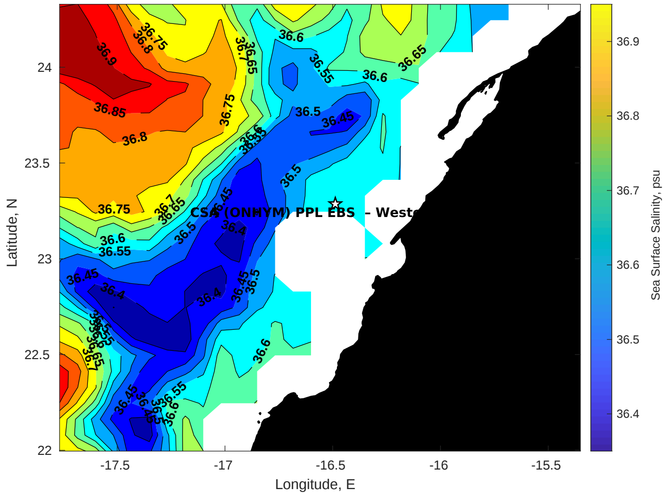
Surface Salinity for CSA (ONHYM) PPL EBS - Western Sahara at 22-Jan-2026 00:00:00
