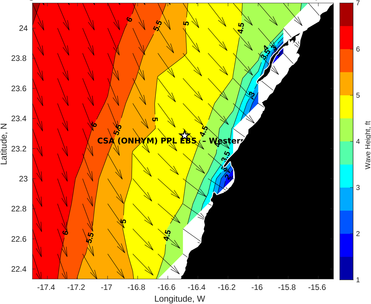
GFS Wave Height (ft) for CSA (ONHYM) PPL EBS - Western Sahara at 23-Jan-2026 09:00:00
