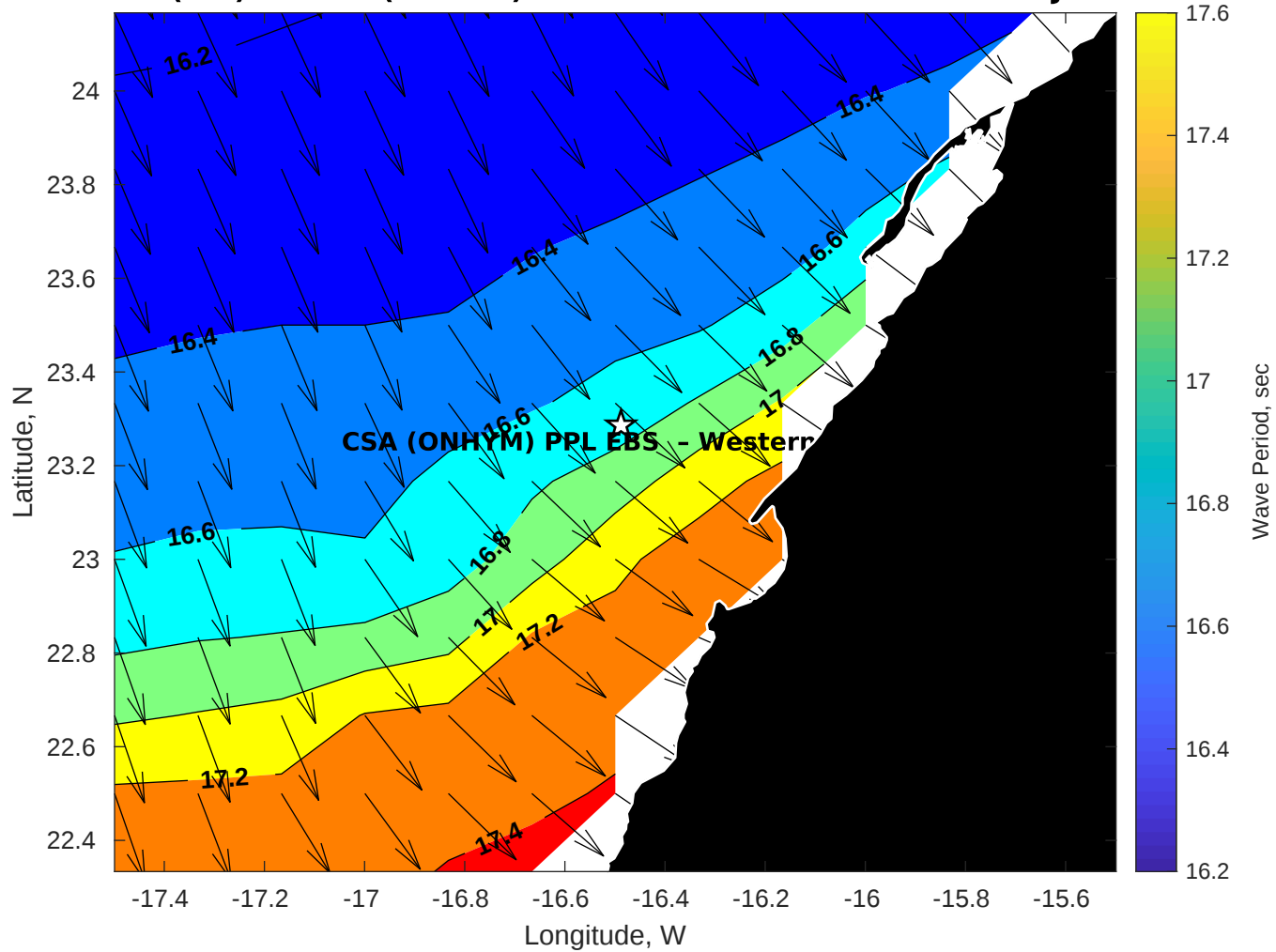
GFS Wave Period (sec) for CSA (ONHYM) PPL EBS - Western Sahara at 23-Jan-2026 09:00:00
