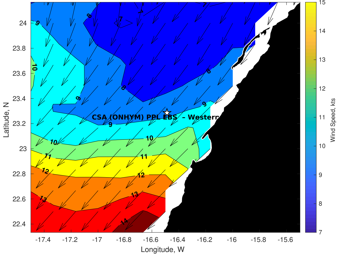
GFS Winds (kts) for CSA (ONHYM) PPL EBS - Western Sahara at 23-Jan-2026 09:00:00
