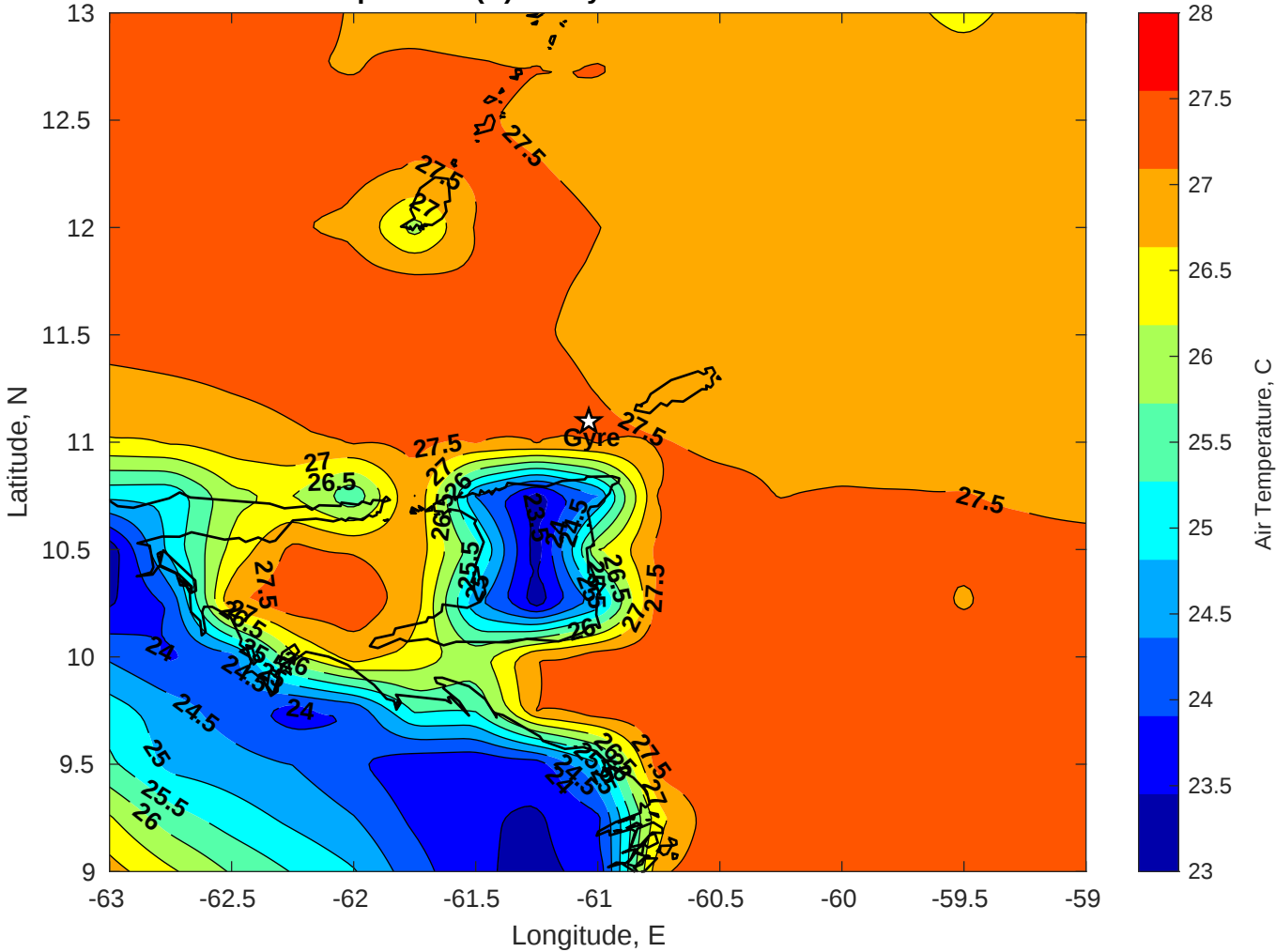
Air Temperature (C) for Gyre at 23-Jan-2026
