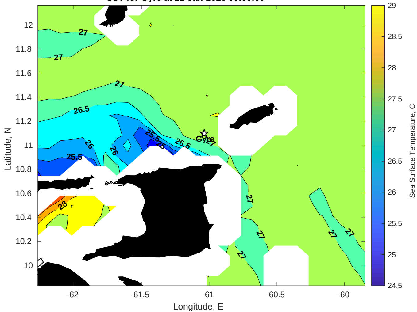
SST for Gyre at 22-Jan-2026 00:00:00
