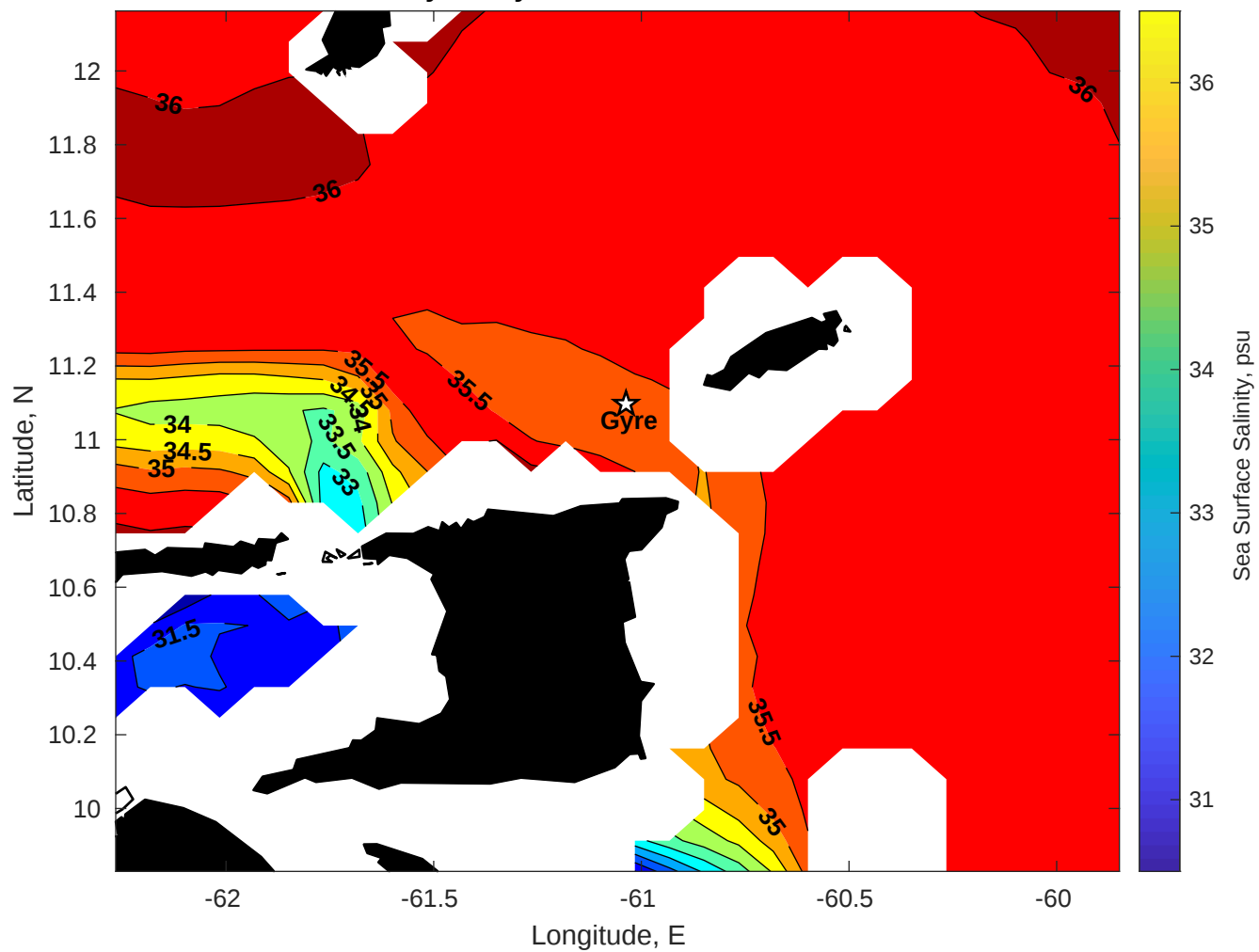
Surface Salinity for Gyre at 22-Jan-2026 00:00:00
