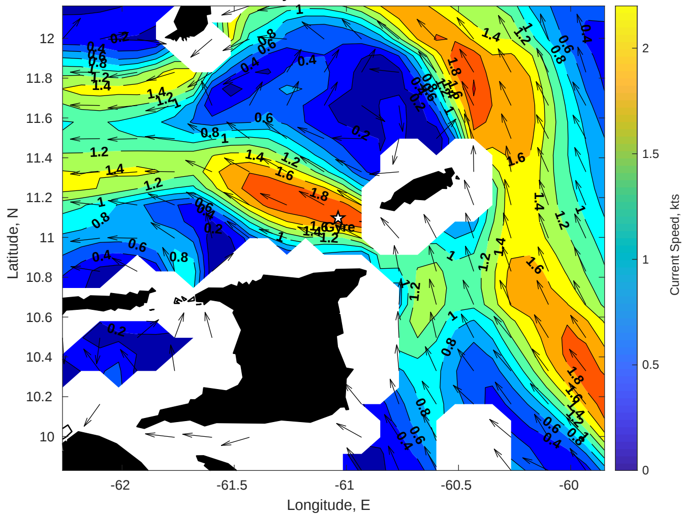
Surface Currents for Gyre at 22-Jan-2026 00:00:00
