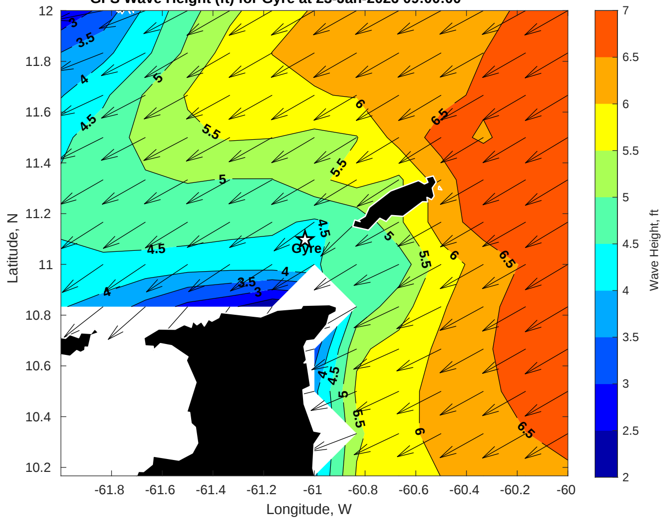
GFS Wave Height (ft) for Gyre at 23-Jan-2026 09:00:00
