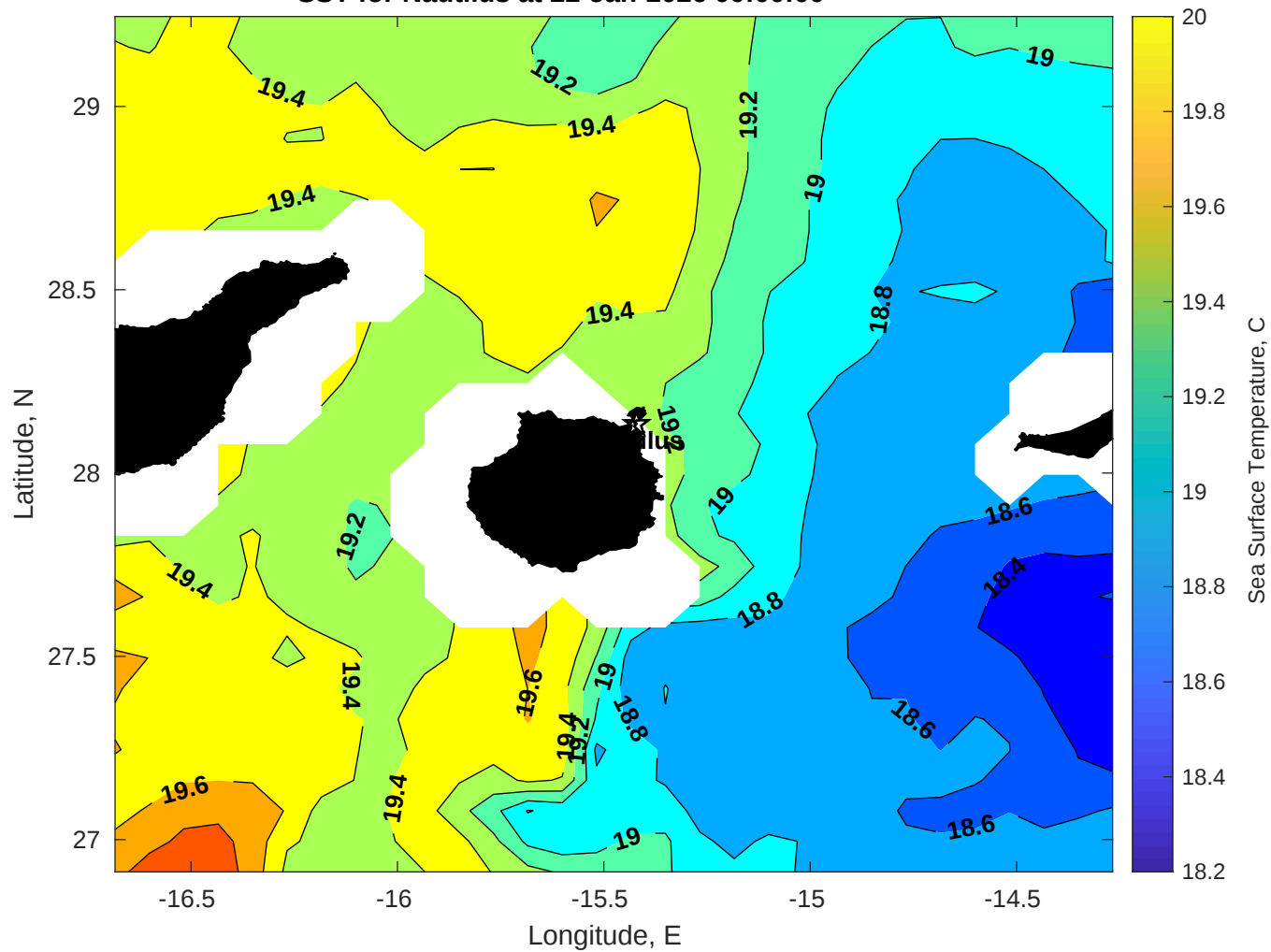
SST for Nautilus at 22-Jan-2026 00:00:00
