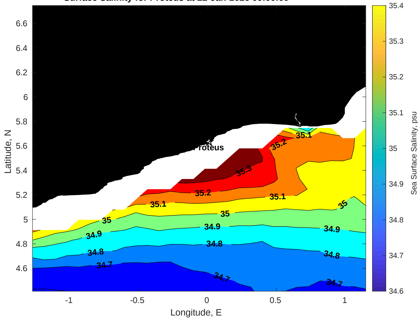
Surface Salinity for Proteus at 22-Jan-2026 00:00:00
