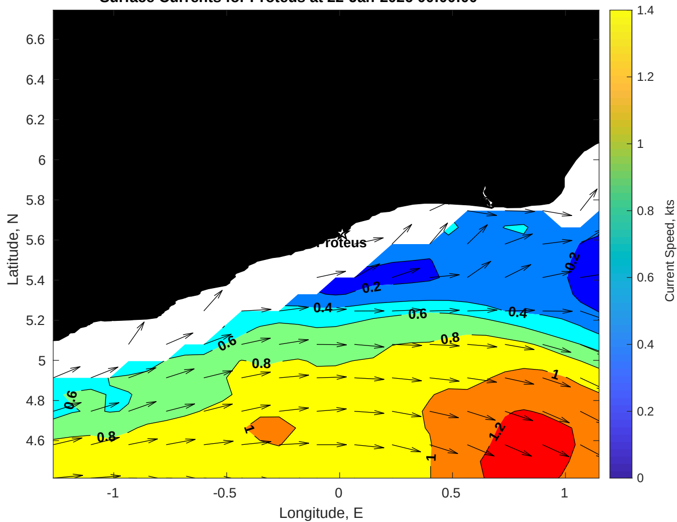
Surface Currents for Proteus at 22-Jan-2026 00:00:00
