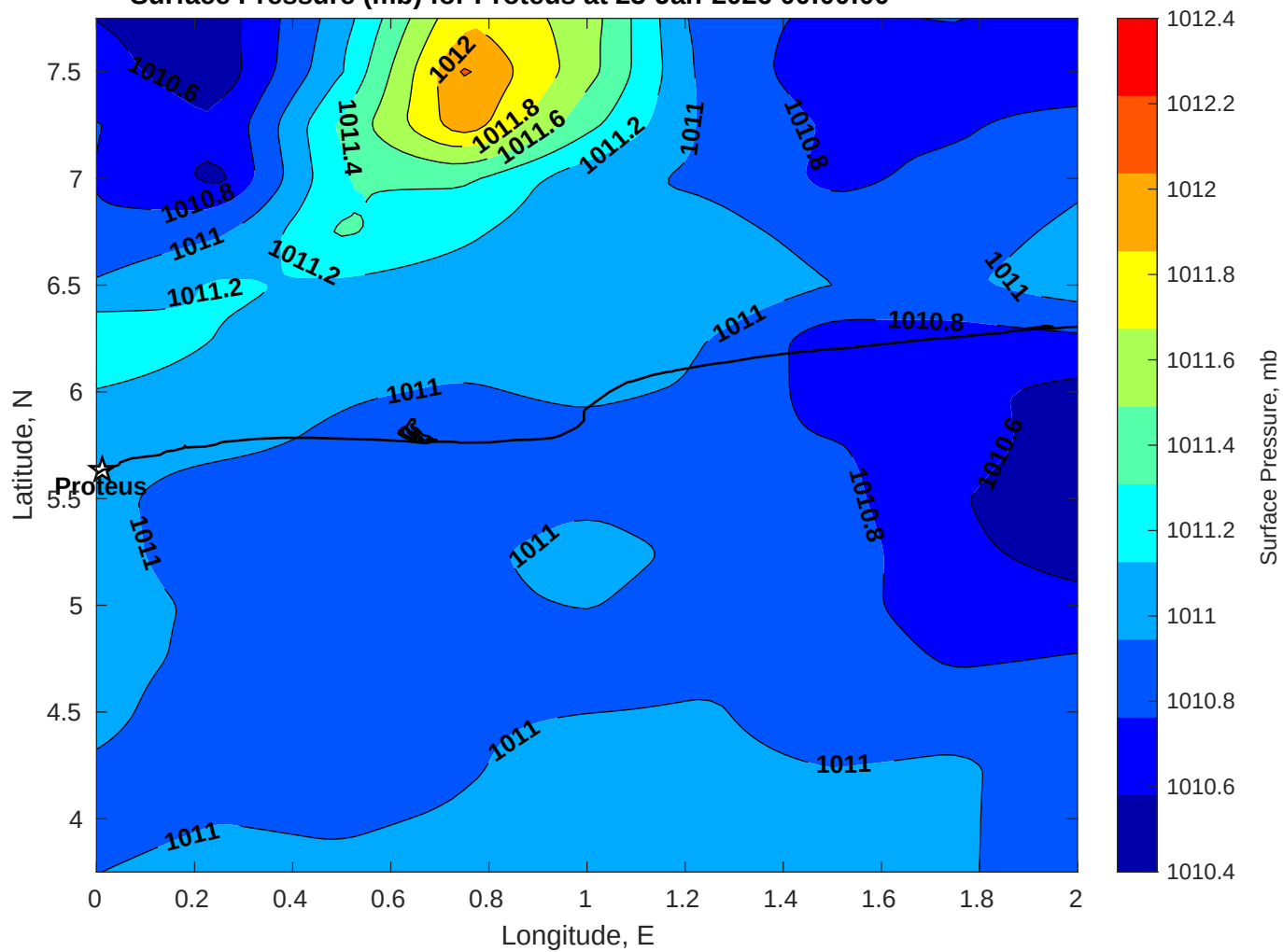
Surface Pressure (mb) for Proteus at 23-Jan-2026 00:00:00
