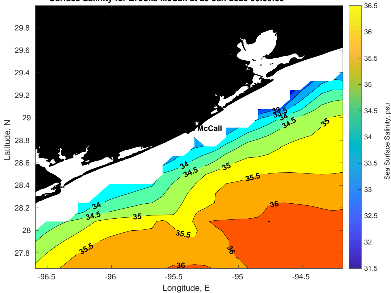
Surface Salinity for Brooks McCall at 23-Jan-2026 00:00:00
