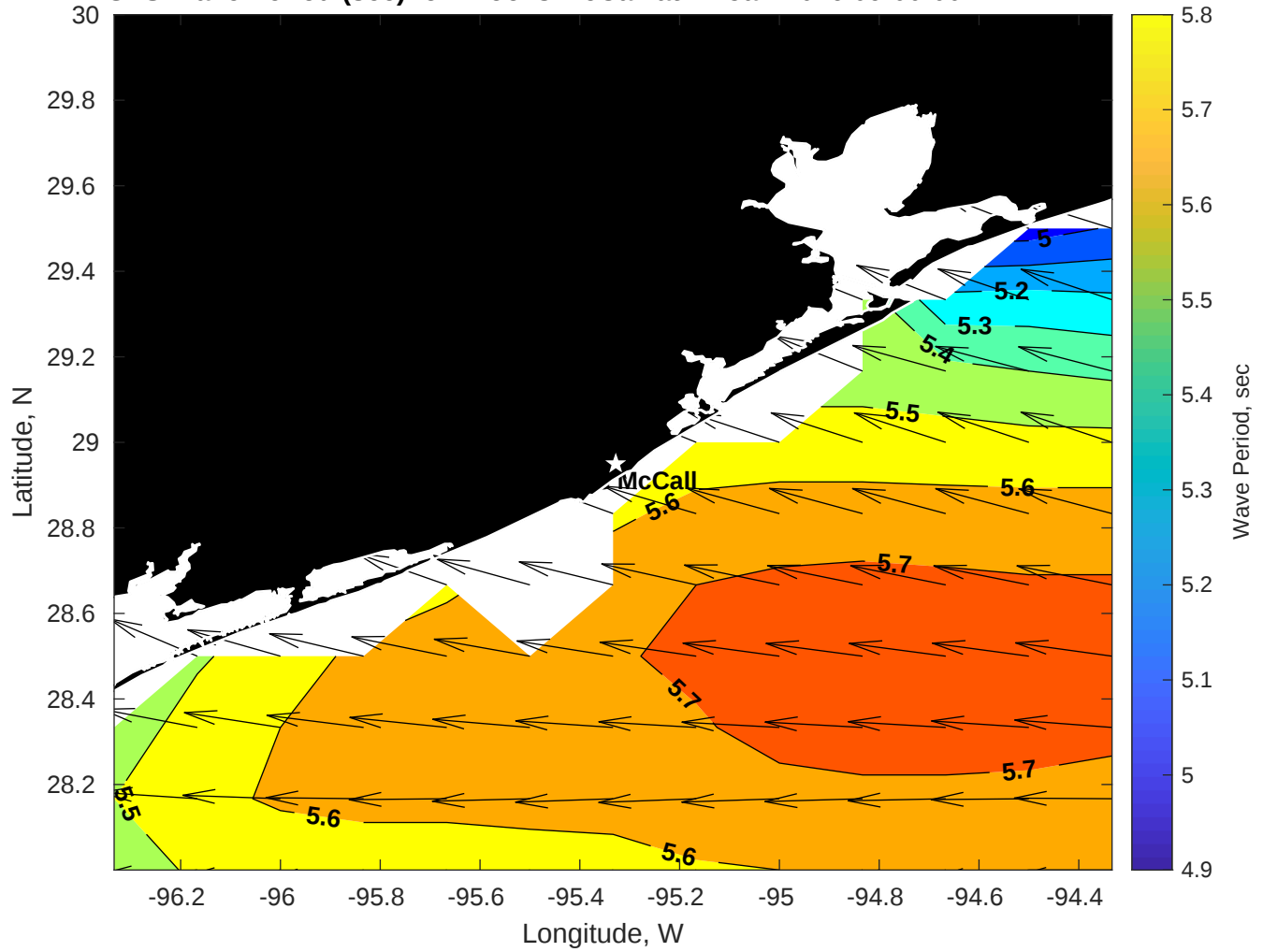
GFS Wave Period (sec) for Brooks McCall at 24-Jan-2026 09:00:00
