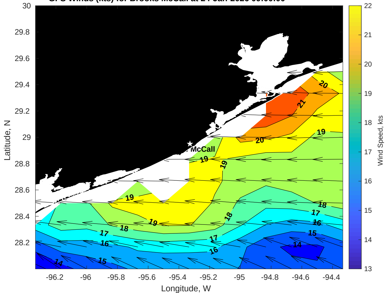
GFS Winds (kts) for Brooks McCall at 24-Jan-2026 09:00:00
