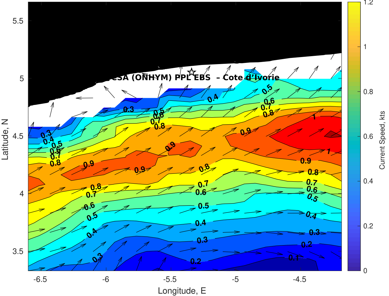
Surface Currents for CSA (ONHYM) PPL EBS - Cote d'Ivoire at 23-Jan-2026 00:00:00
