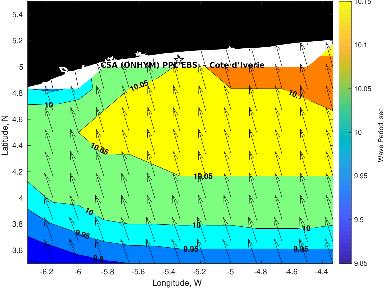
GFS Wave Period (sec) for CSA (ONHYM) PPL EBS - Cote d'Ivoire at 24-Jan-2026 09:00:00
