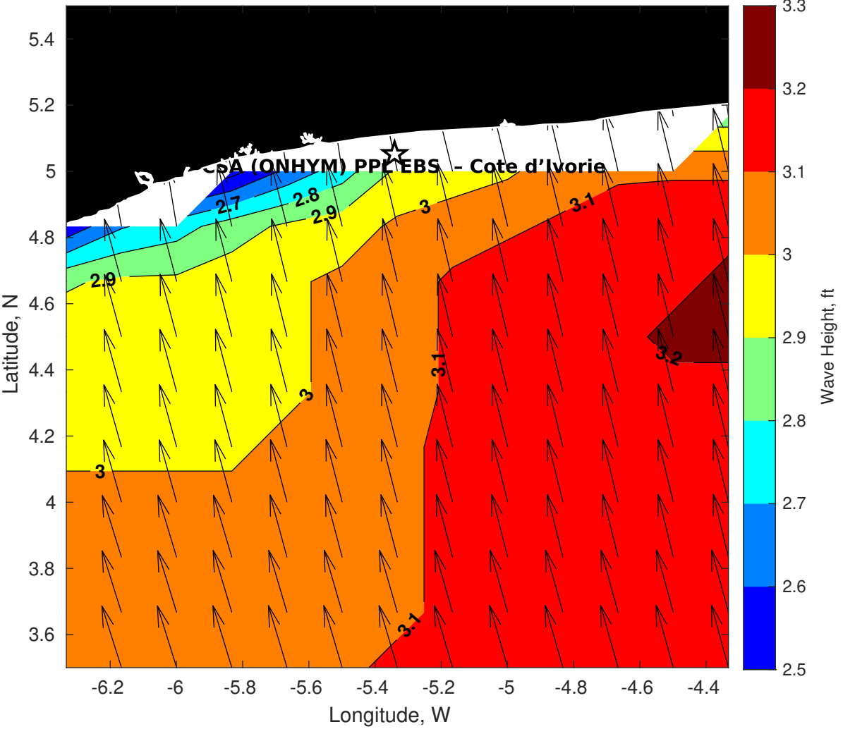
GFS Wave Height (ft) for CSA (ONHYM) PPL EBS - Cote d'Ivoire at 24-Jan-2026 09:00:00
