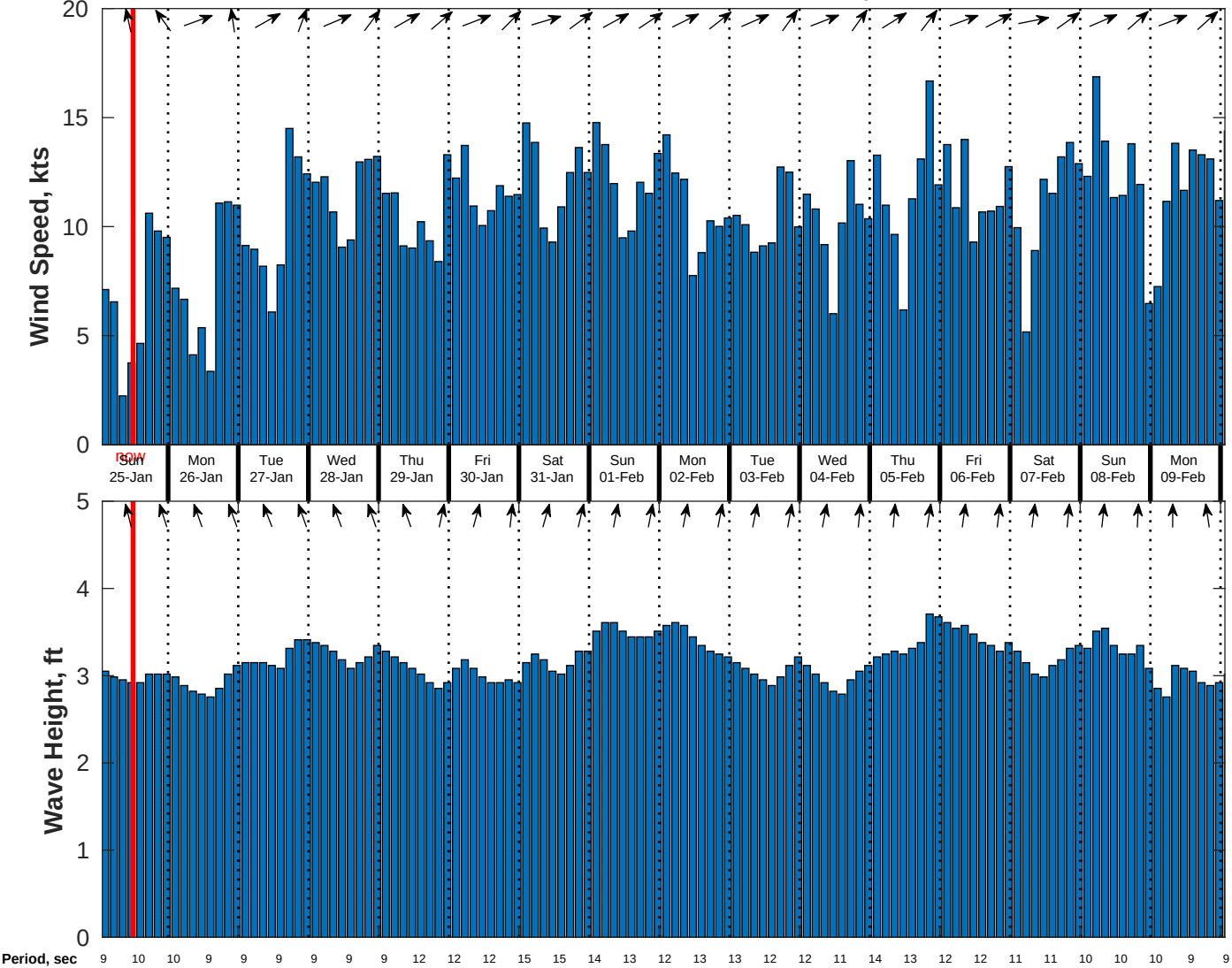
Wind & Wave Forecast for CSA (ONHYM) PPL EBS - Cote d'Ivoire from 24-Jan-2026 01:00:00 to 09-Feb-2026 01:00:00
