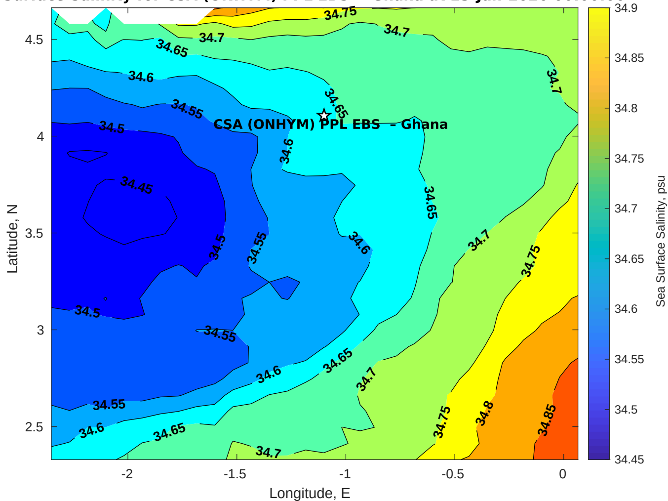
Surface Salinity for CSA (ONHYM) PPL EBS - Ghana at 23-Jan-2026 00:00:00
