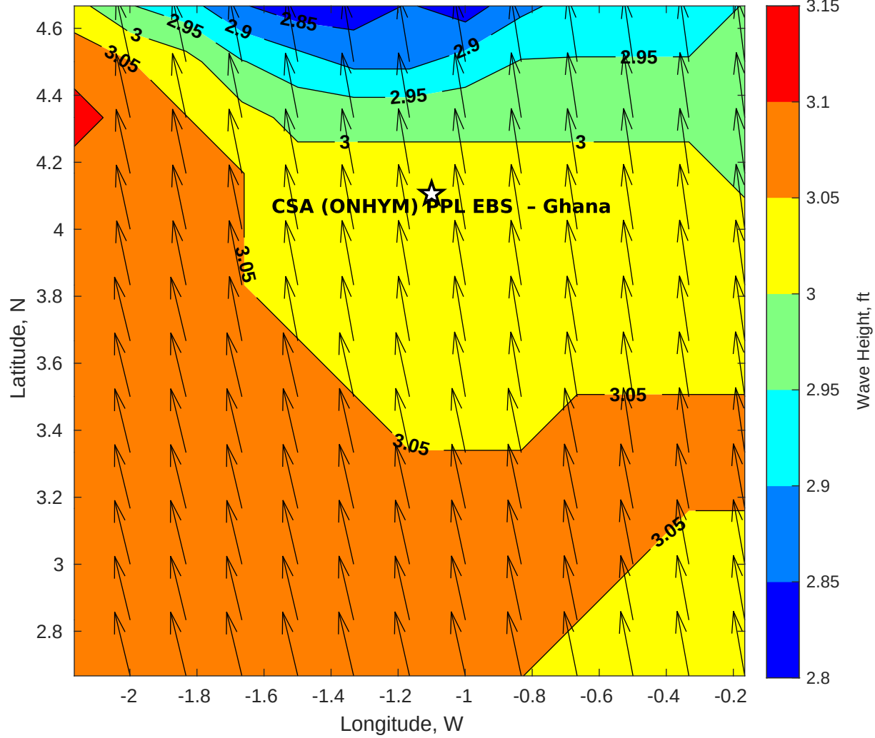
GFS Wave Height (ft) for CSA (ONHYM) PPL EBS - Ghana at 24-Jan-2026 09:00:00
