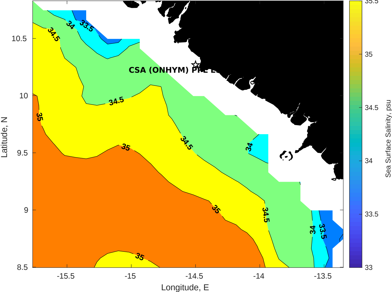
Surface Salinity for CSA (ONHYM) PPL EBS - Guinea at 23-Jan-2026 00:00:00
