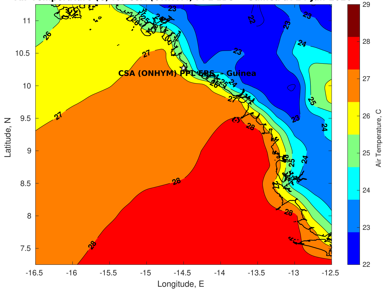
Air Temperature (C) for CSA (ONHYM) PPL EBS - Guinea at 24-Jan-2026
