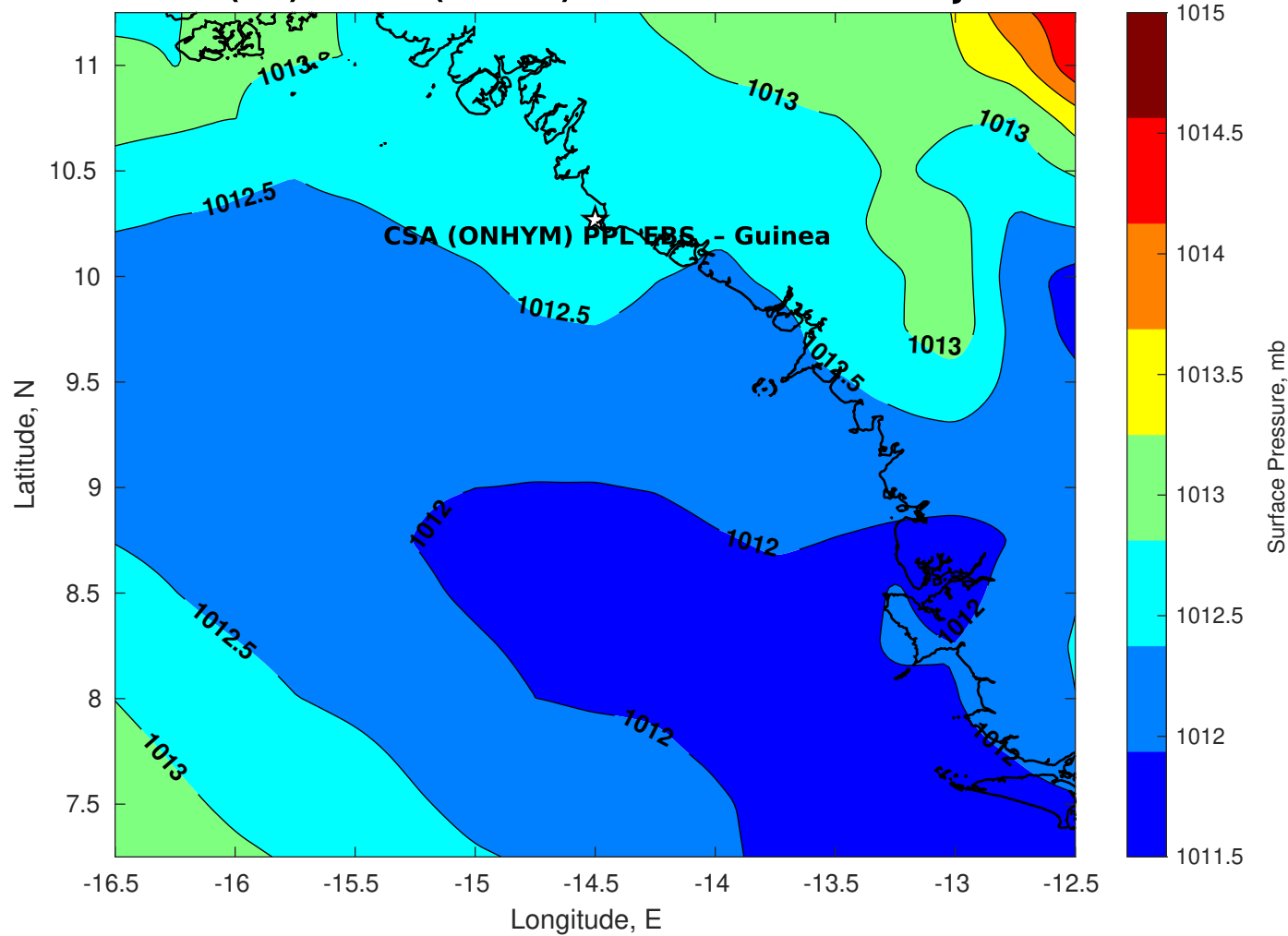
Surface Pressure (mb) for CSA (ONHYM) PPL EBS - Guinea at 26-Jan-2026 00:00:00
