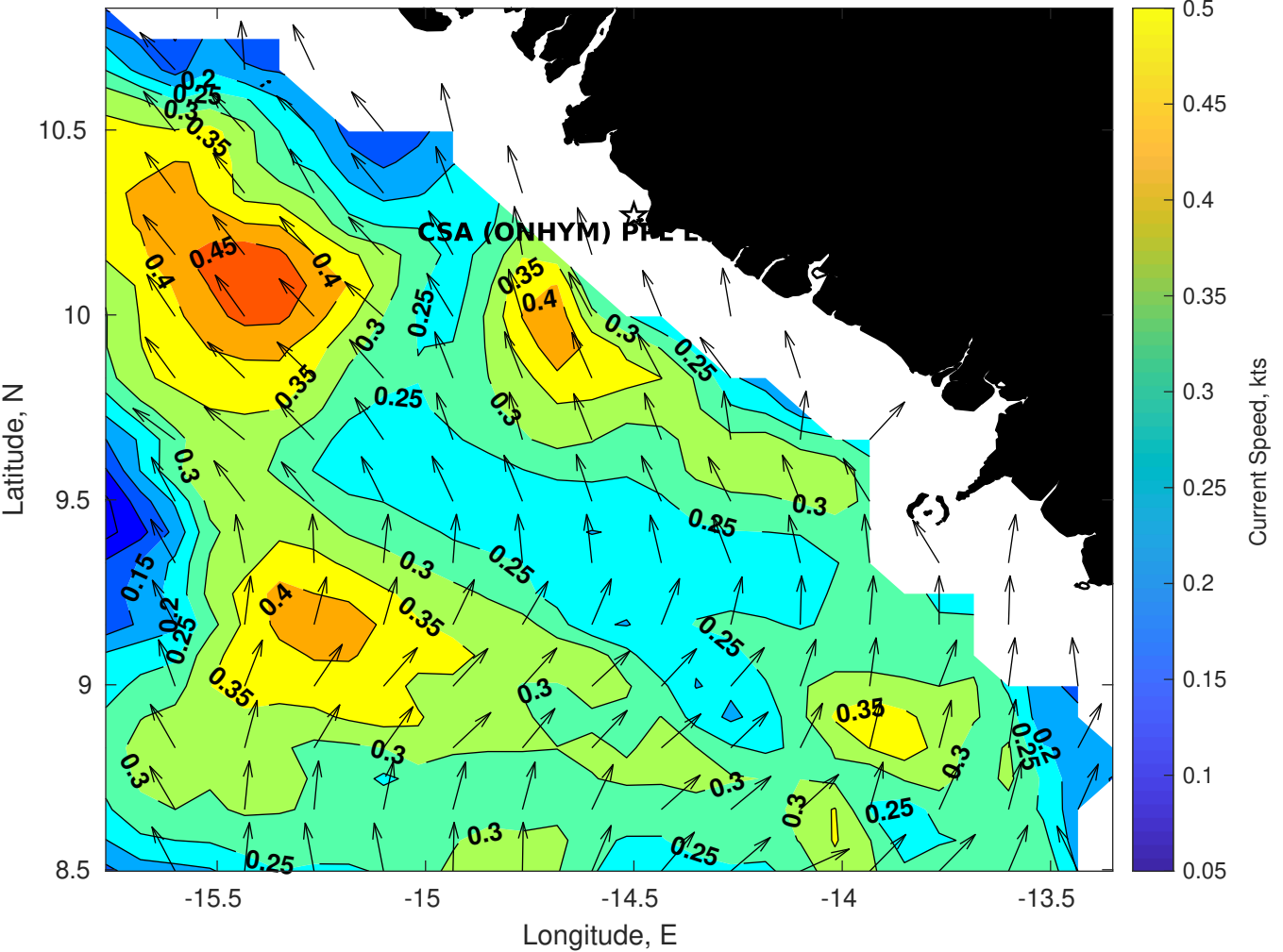
Surface Currents for CSA (ONHYM) PPL EBS - Guinea at 23-Jan-2026 00:00:00
