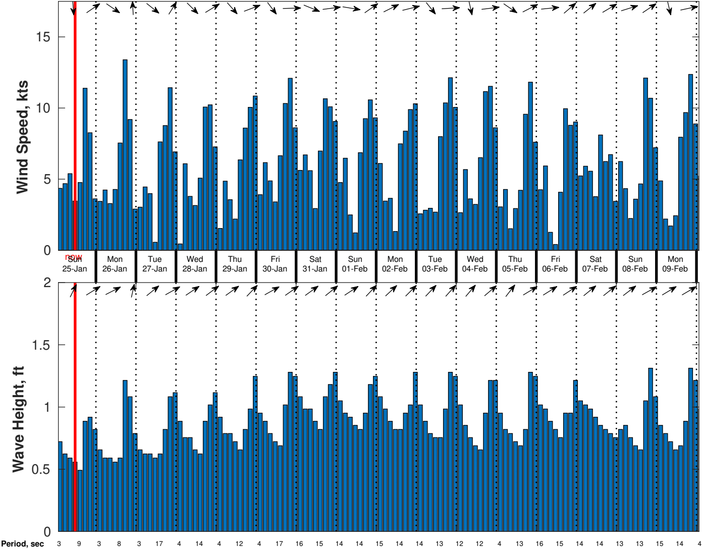
Wind & Wave Forecast for CSA (ONHYM) PPL EBS - Guinea from 24-Jan-2026 01:00:00 to 09-Feb-2026 01:00:00
