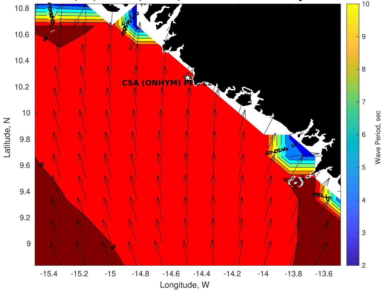
GFS Wave Period (sec) for CSA (ONHYM) PPL EBS - Guinea at 24-Jan-2026 09:00:00
