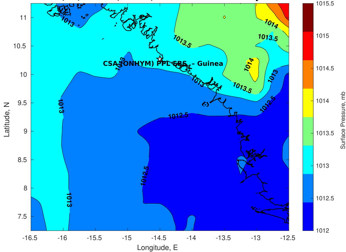
Surface Pressure (mb) for CSA (ONHYM) PPL EBS - Guinea at 24-Jan-2026 00:00:00
