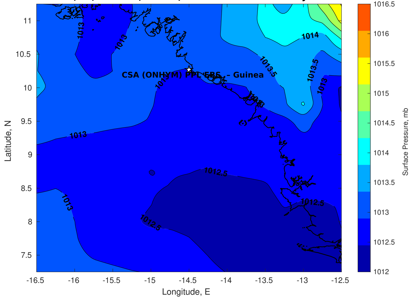
Surface Pressure (mb) for CSA (ONHYM) PPL EBS - Guinea at 25-Jan-2026 00:00:00
