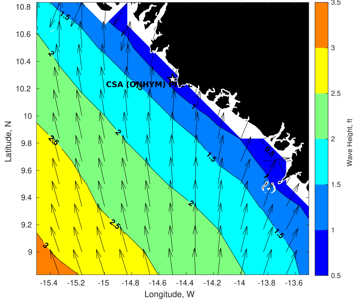
GFS Wave Height (ft) for CSA (ONHYM) PPL EBS - Guinea at 24-Jan-2026 09:00:00
