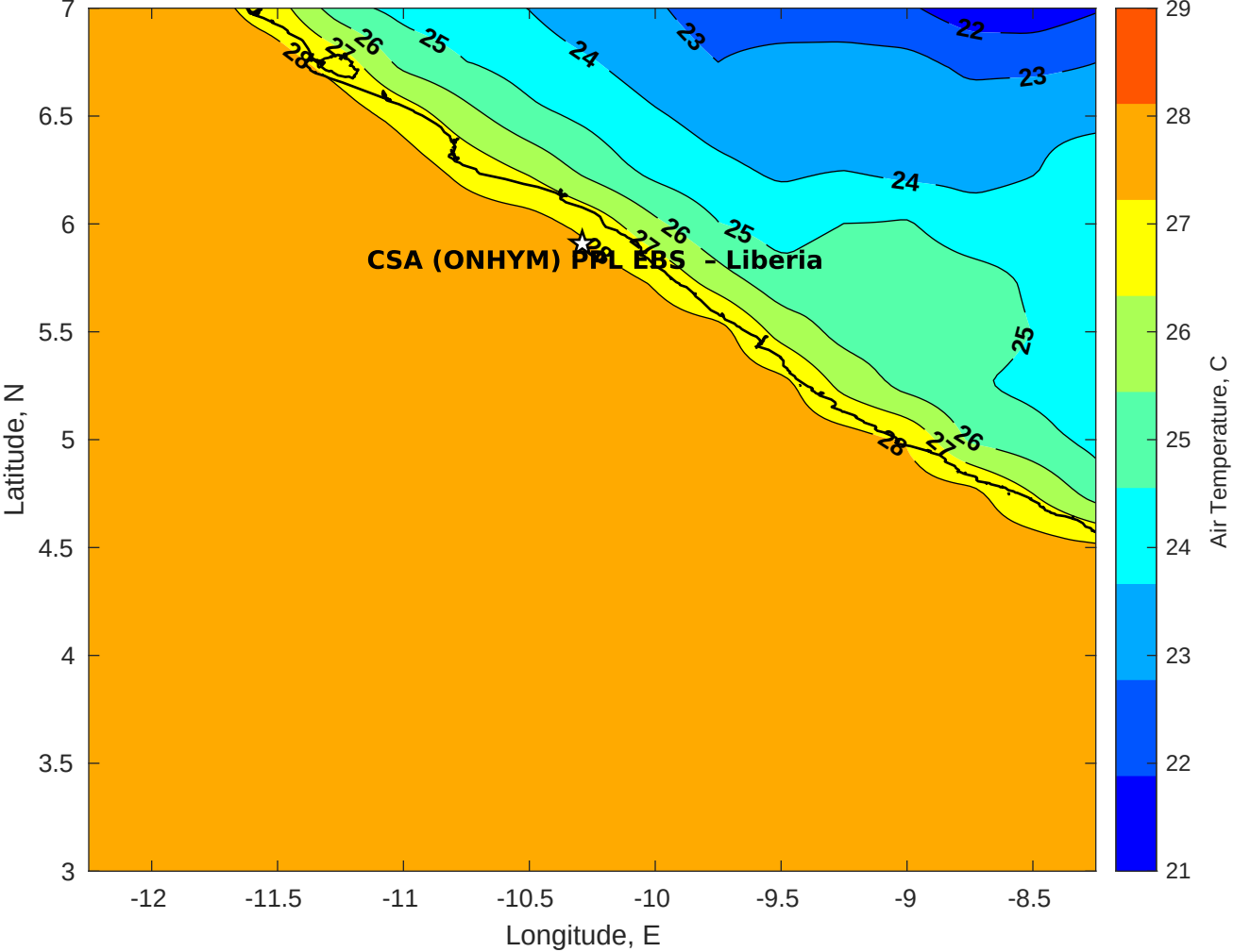
Air Temperature (C) for CSA (ONHYM) PPL EBS - Liberia at 24-Jan-2026
