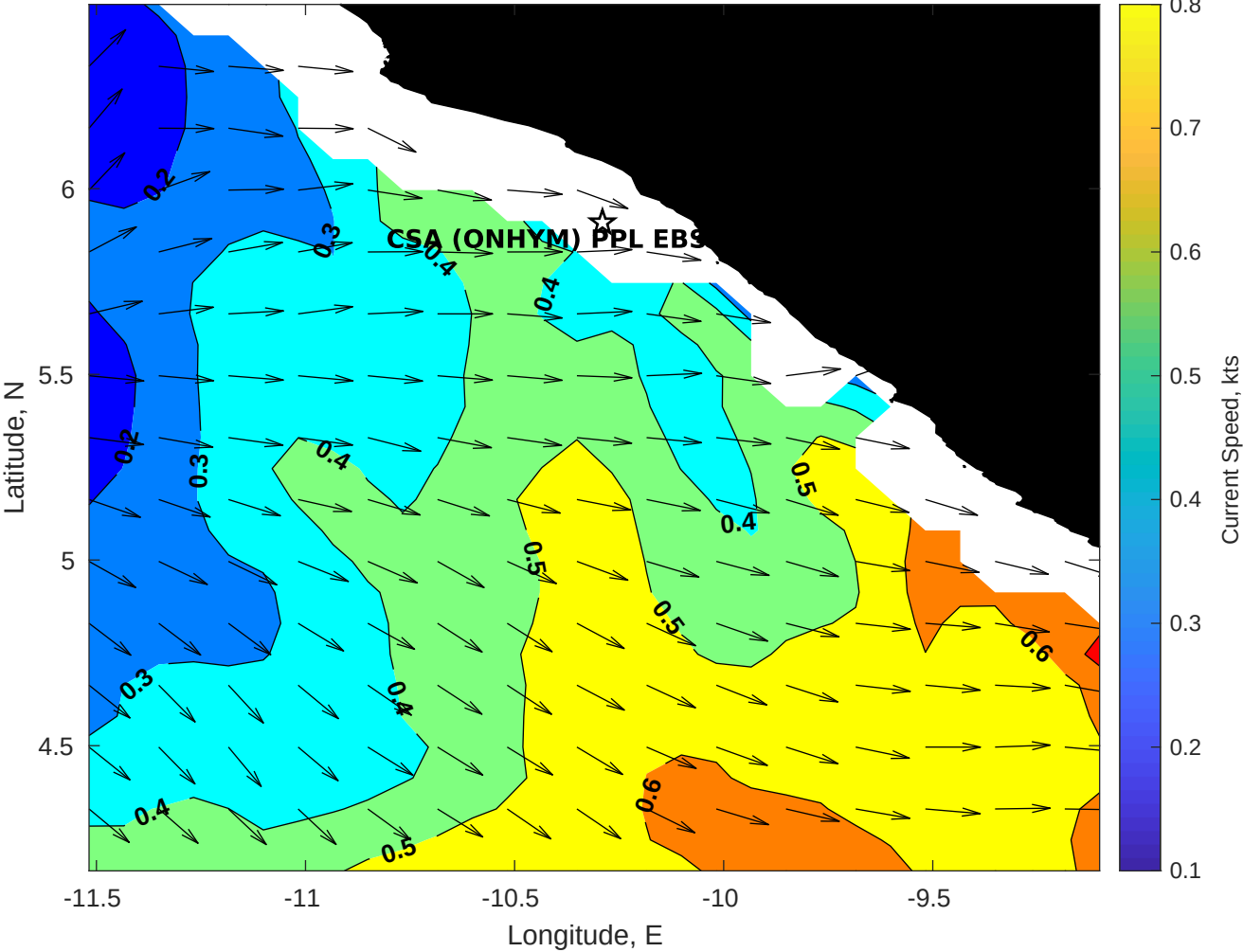
Surface Currents for CSA (ONHYM) PPL EBS - Liberia at 23-Jan-2026 00:00:00
