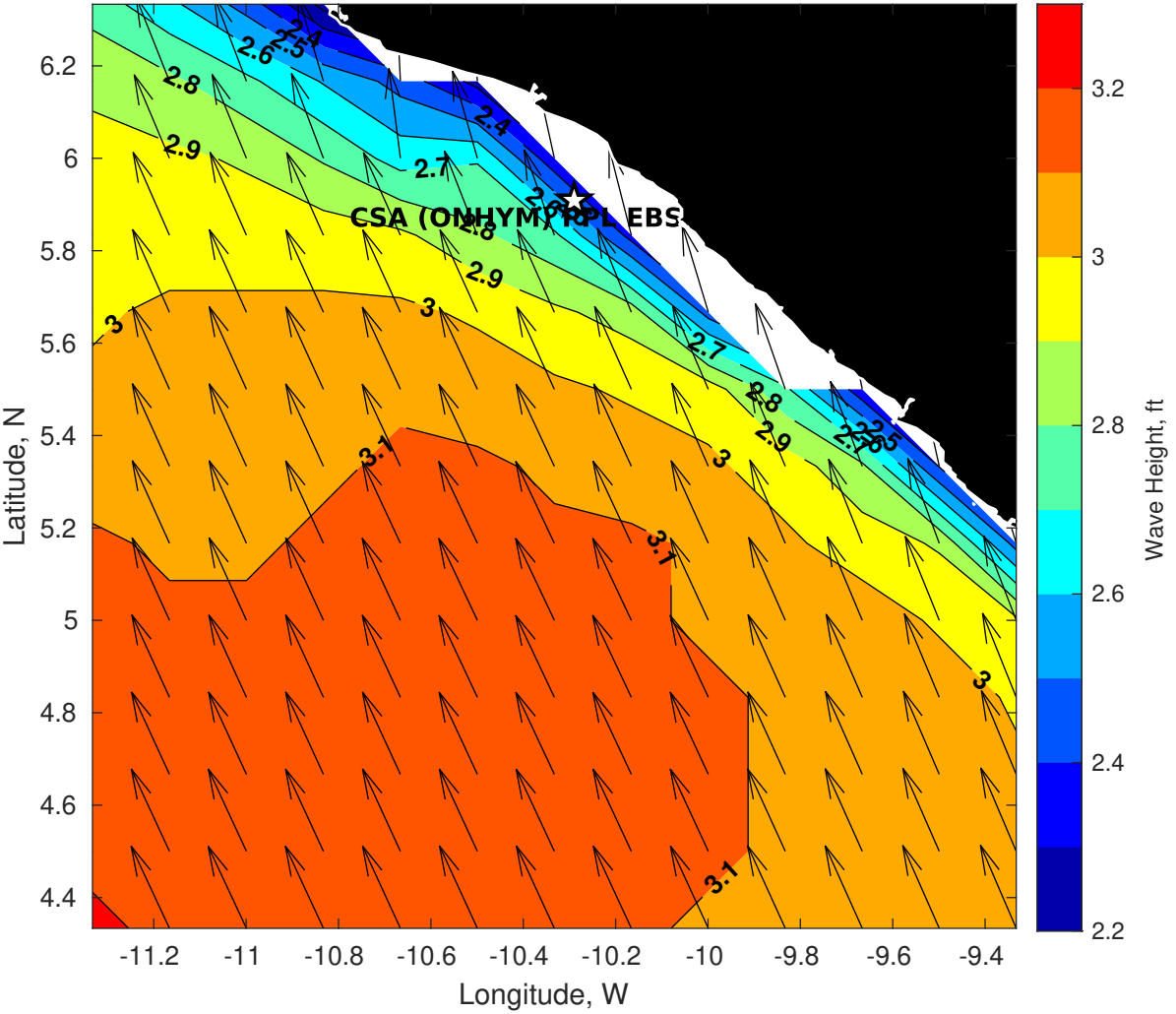
GFS Wave Height (ft) for CSA (ONHYM) PPL EBS - Liberia at 24-Jan-2026 09:00:00
