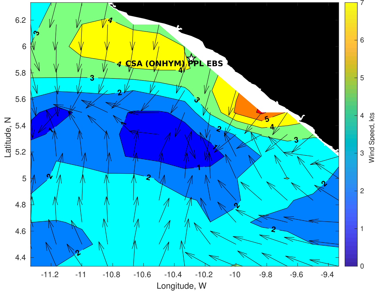
GFS Winds (kts) for CSA (ONHYM) PPL EBS - Liberia at 24-Jan-2026 09:00:00
