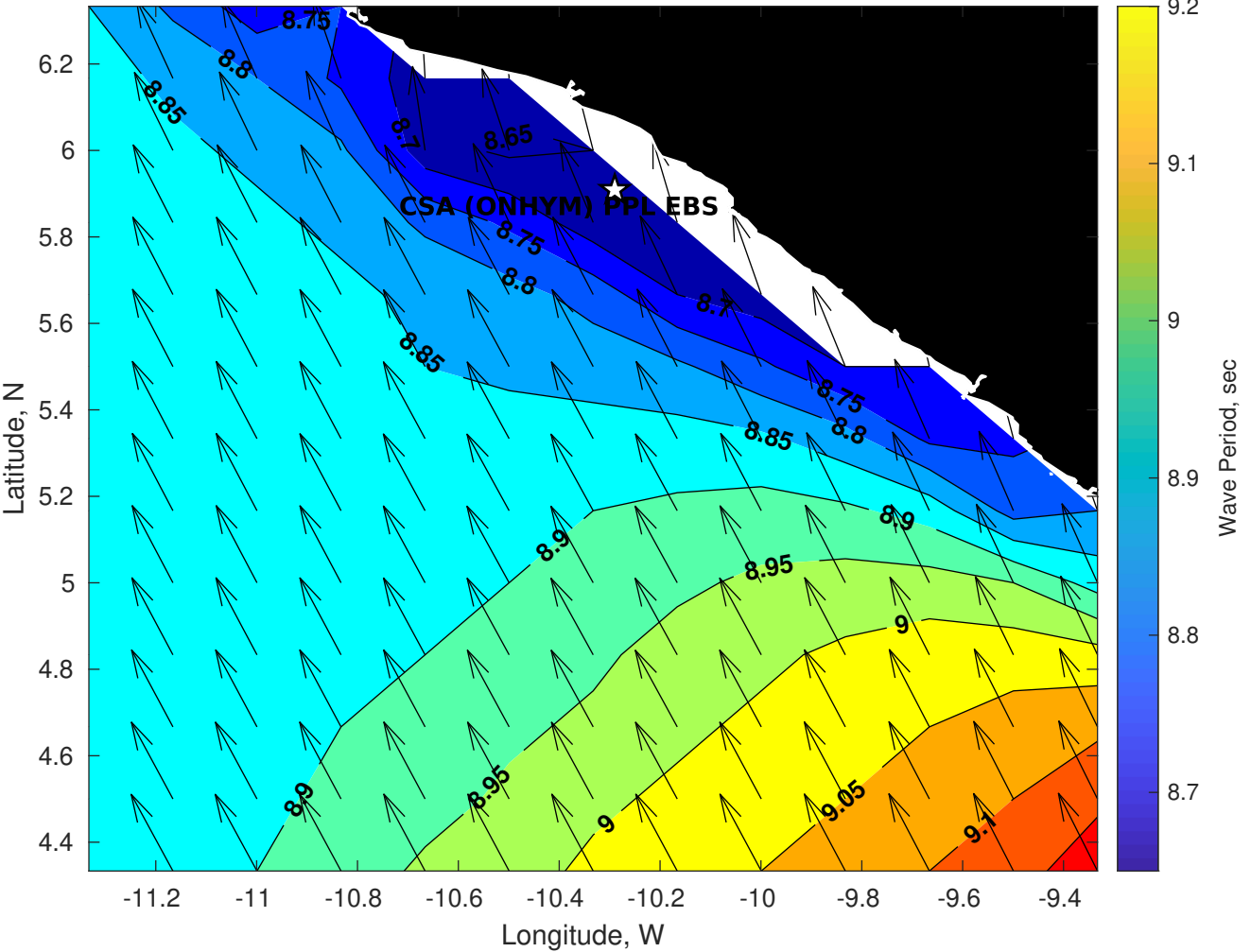
GFS Wave Period (sec) for CSA (ONHYM) PPL EBS - Liberia at 24-Jan-2026 09:00:00
