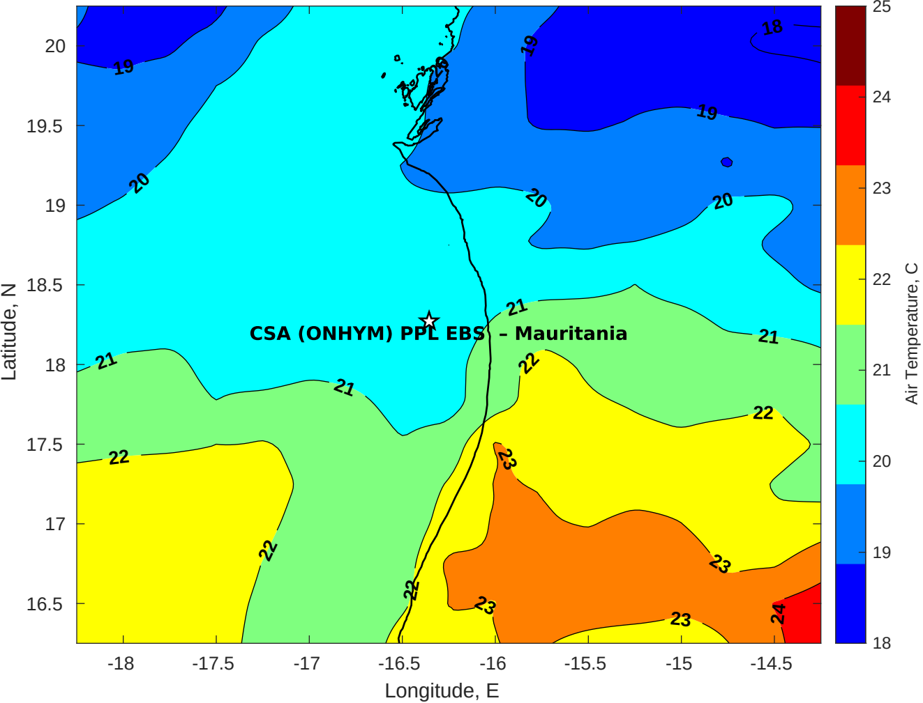
Air Temperature (C) for CSA (ONHYM) PPL EBS - Mauritania at 24-Jan-2026
