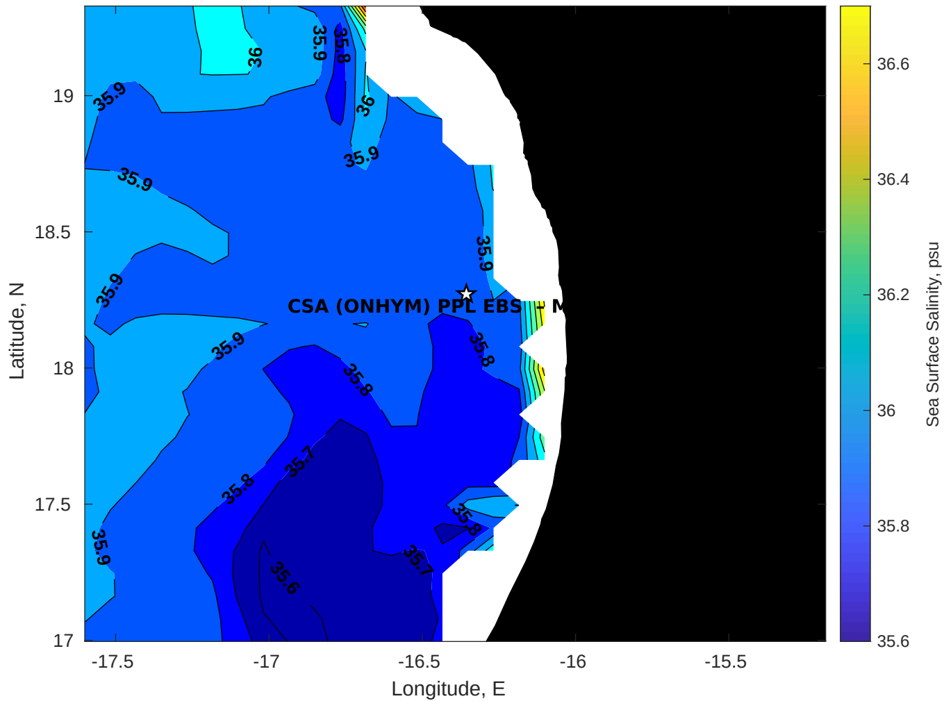
Surface Salinity for CSA (ONHYM) PPL EBS - Mauritania at 23-Jan-2026 00:00:00
