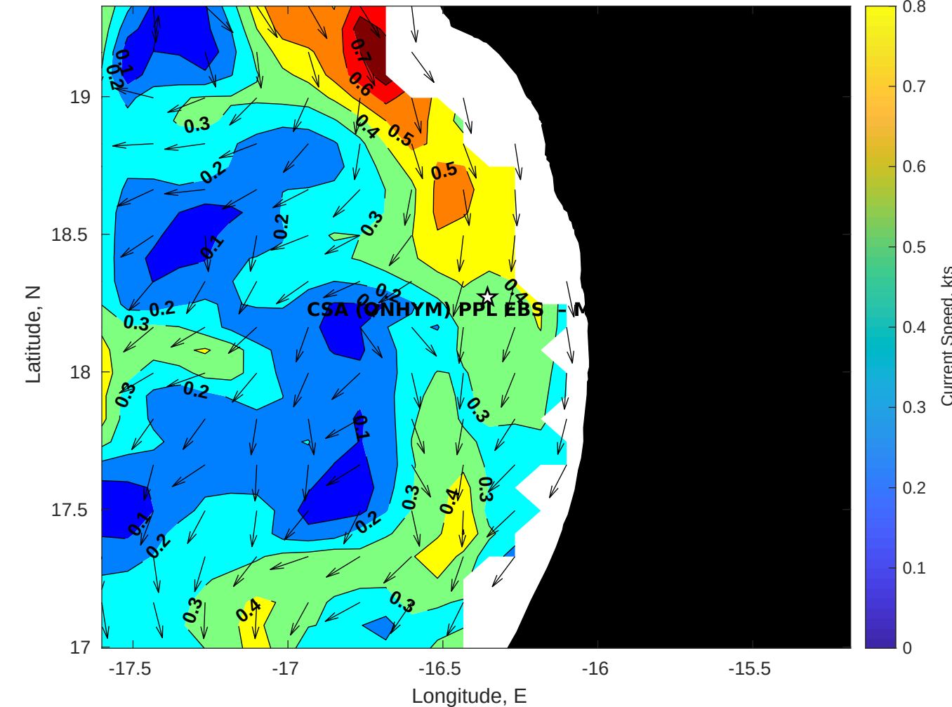
Surface Currents for CSA (ONHYM) PPL EBS - Mauritania at 23-Jan-2026 00:00:00
