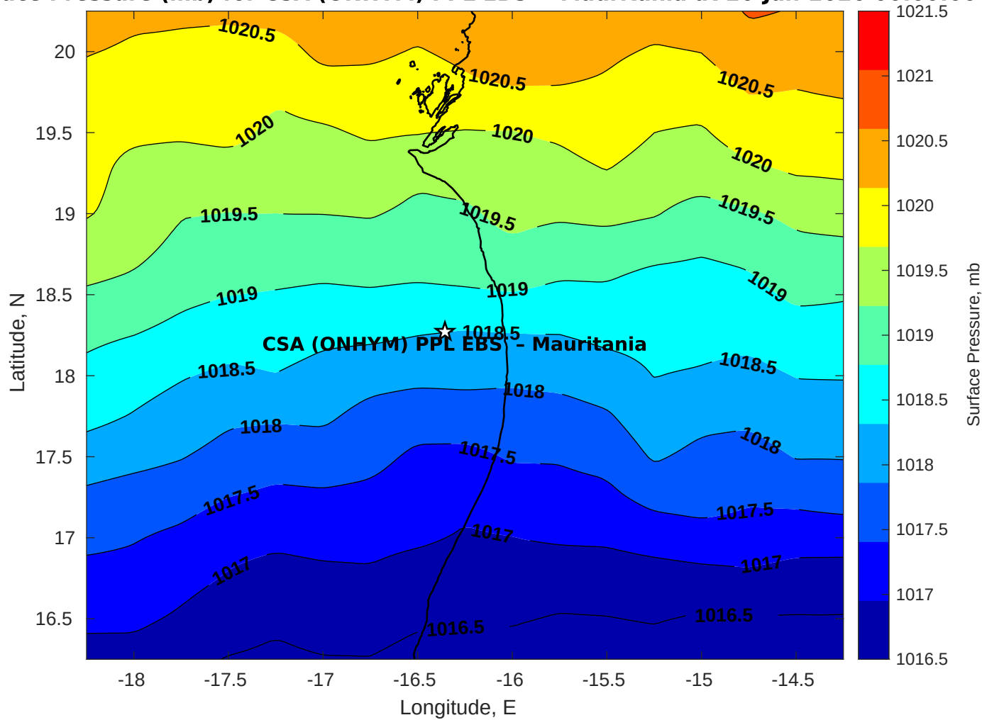
Surface Pressure (mb) for CSA (ONHYM) PPL EBS - Mauritania at 26-Jan-2026 00:00:00
