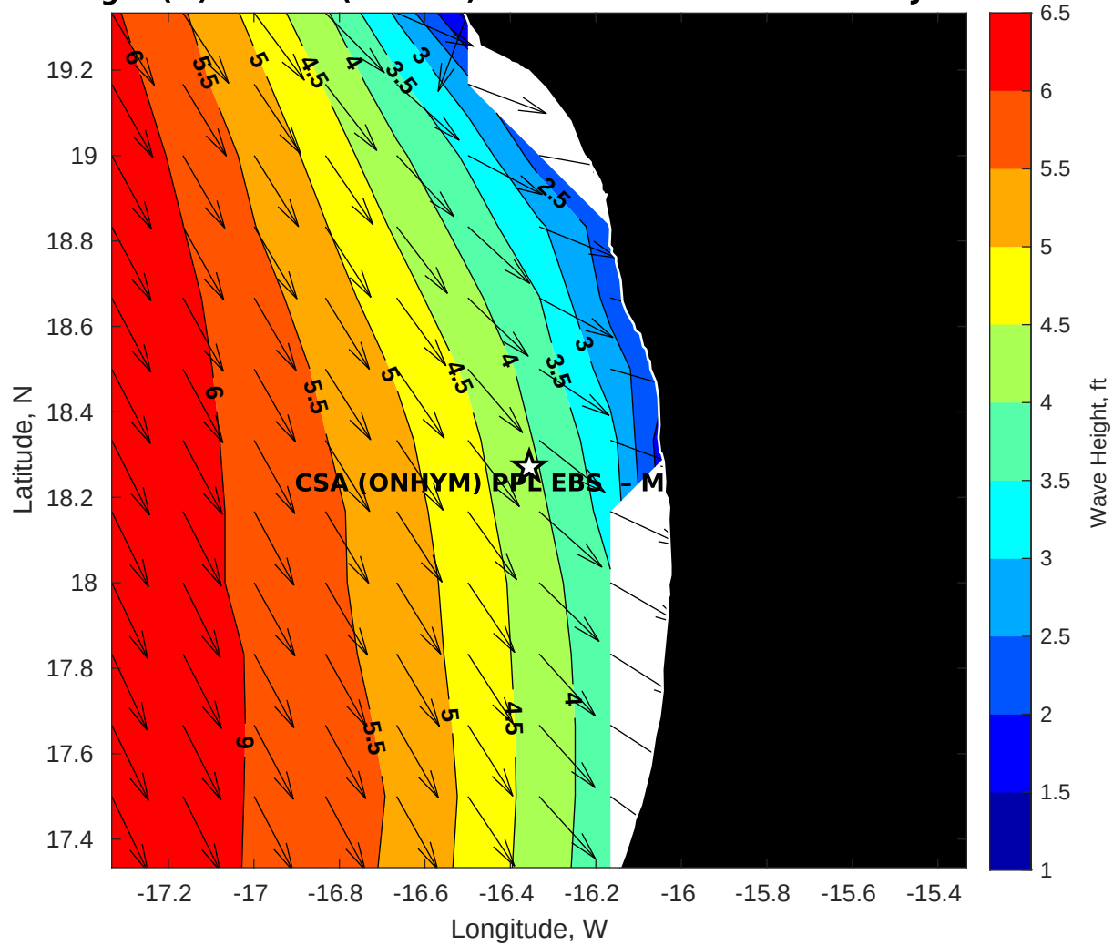
GFS Wave Height (ft) for CSA (ONHYM) PPL EBS - Mauritania at 24-Jan-2026 09:00:00
