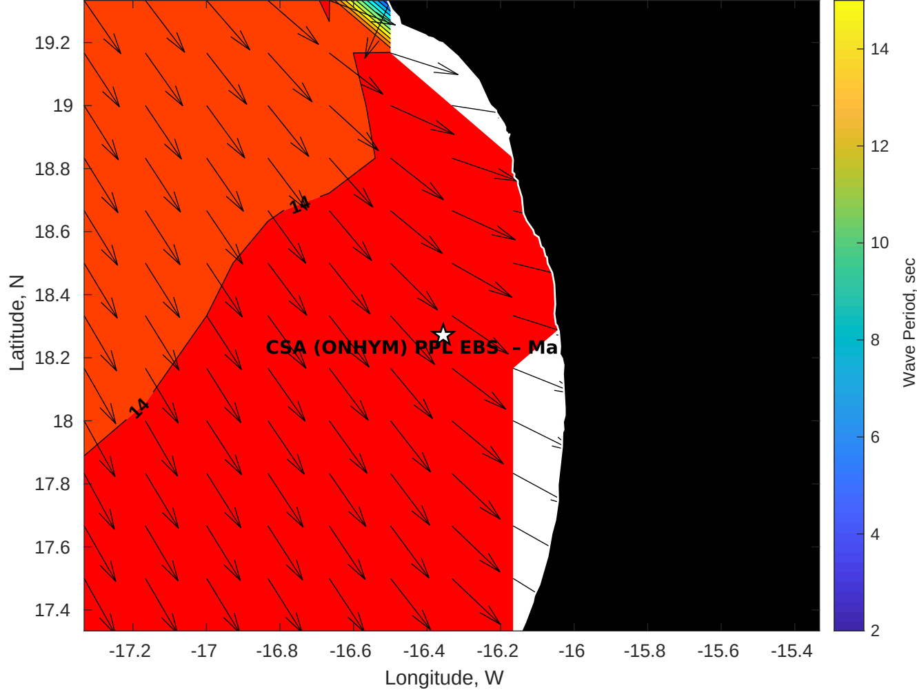
GFS Wave Period (sec) for CSA (ONHYM) PPL EBS - Mauritania at 24-Jan-2026 09:00:00
