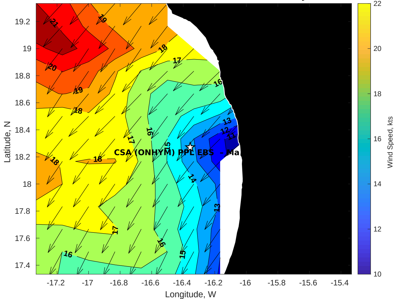
GFS Winds (kts) for CSA (ONHYM) PPL EBS - Mauritania at 24-Jan-2026 09:00:00
