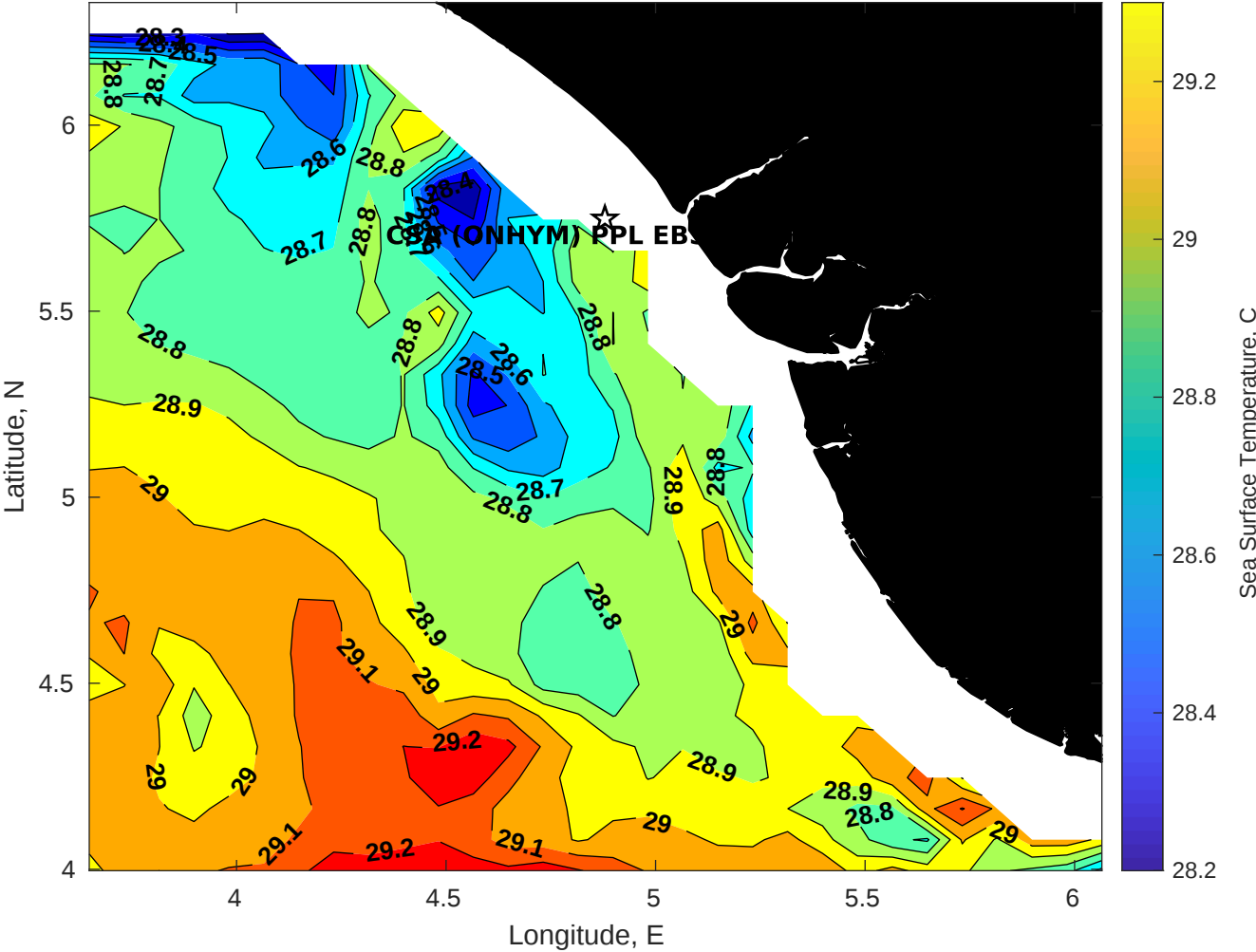
SST for CSA (ONHYM) PPL EBS - Nigeria at 23-Jan-2026 00:00:00
