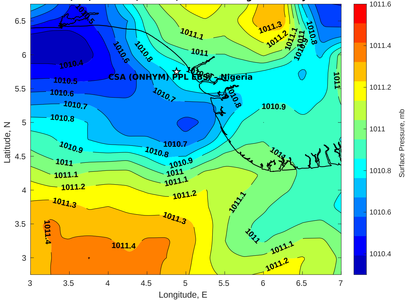
Surface Pressure (mb) for CSA (ONHYM) PPL EBS - Nigeria at 19-Jul-2031 00:00:00
