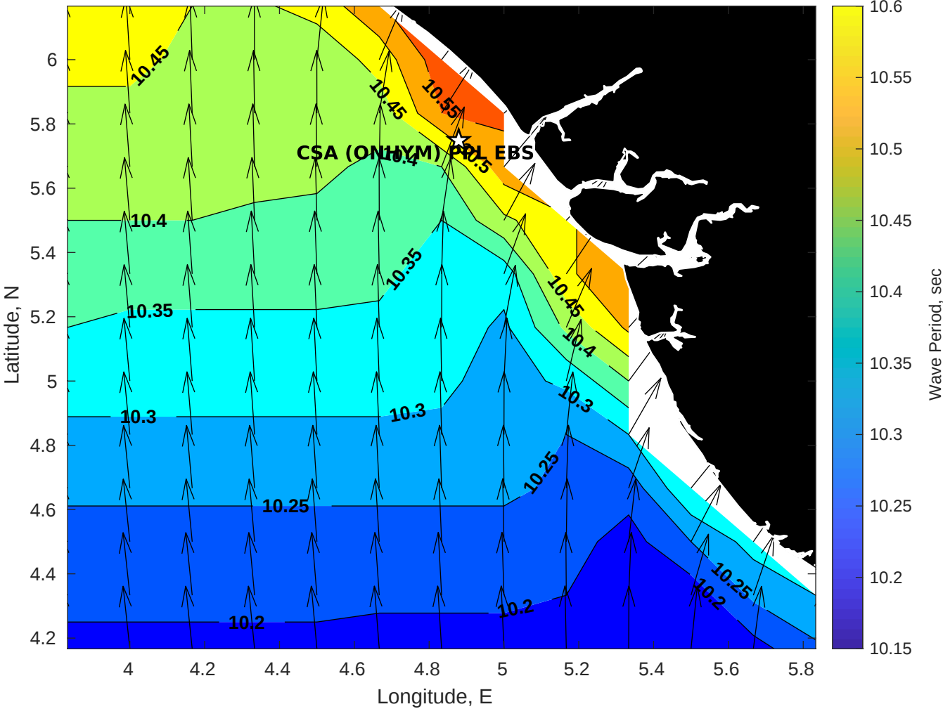
GFS Wave Period (sec) for CSA (ONHYM) PPL EBS - Nigeria at 24-Jan-2026 09:00:00
