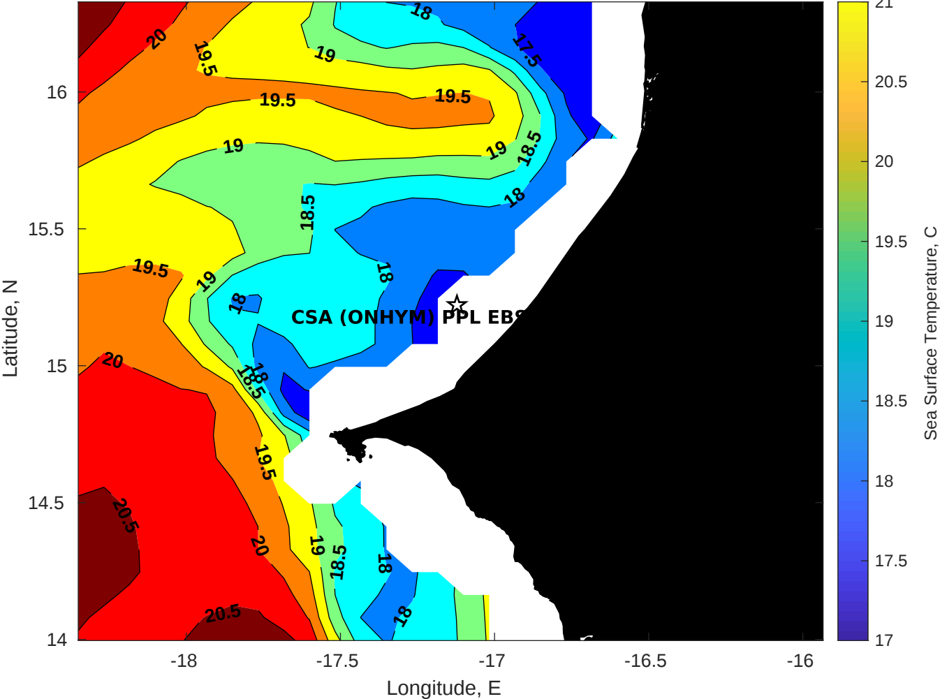
SST for CSA (ONHYM) PPL EBS - Senegal at 23-Jan-2026 00:00:00
