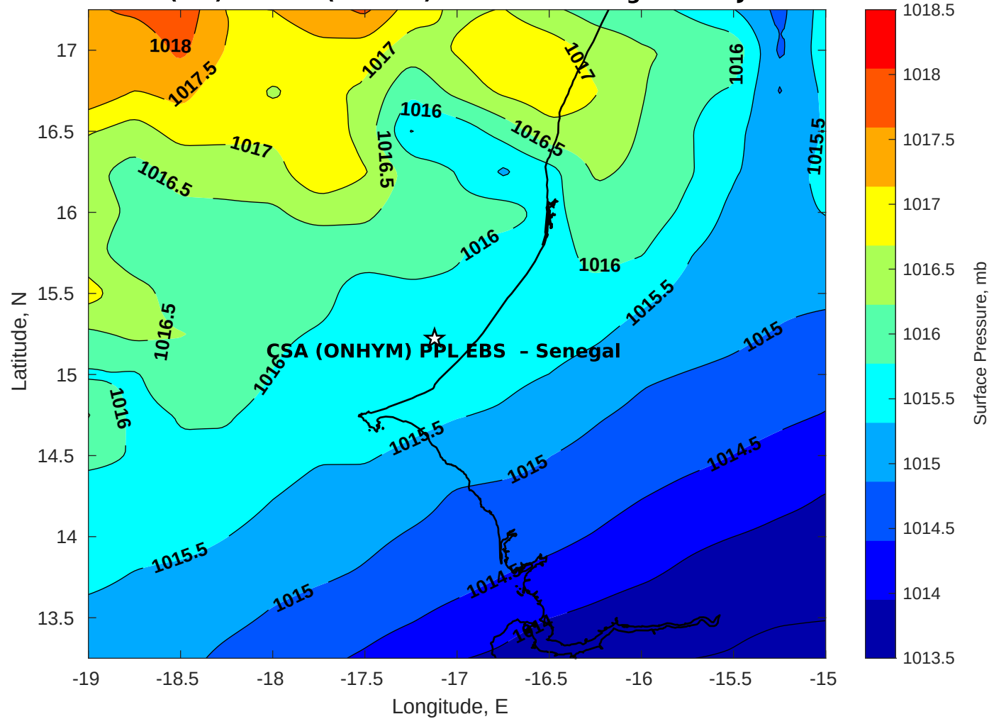
Surface Pressure (mb) for CSA (ONHYM) PPL EBS - Senegal at 24-Jan-2026 00:00:00
